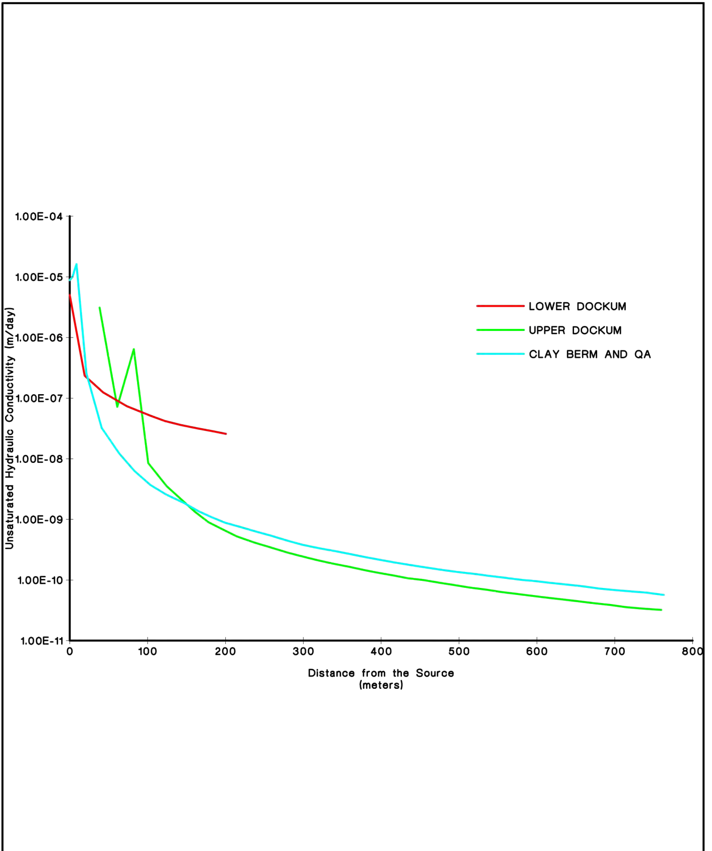
STEADY STATE UNSATURATED HYDRAULIC CONDUCTIVITY vs. DISTANCE FROM SOURCE TRIASSIC PARK WASTE DISPOSAL FACILITY Figure 3-23
