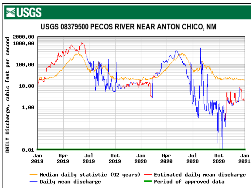
Figure 1.5 Daily discharge in 2019 and 2020 for the Pecos River near Anton Chico, NM.
