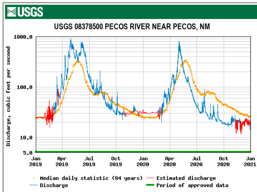
Figure 1.4 Daily discharge in 2019 and 2020 for the Pecos River near Pecos, NM.
