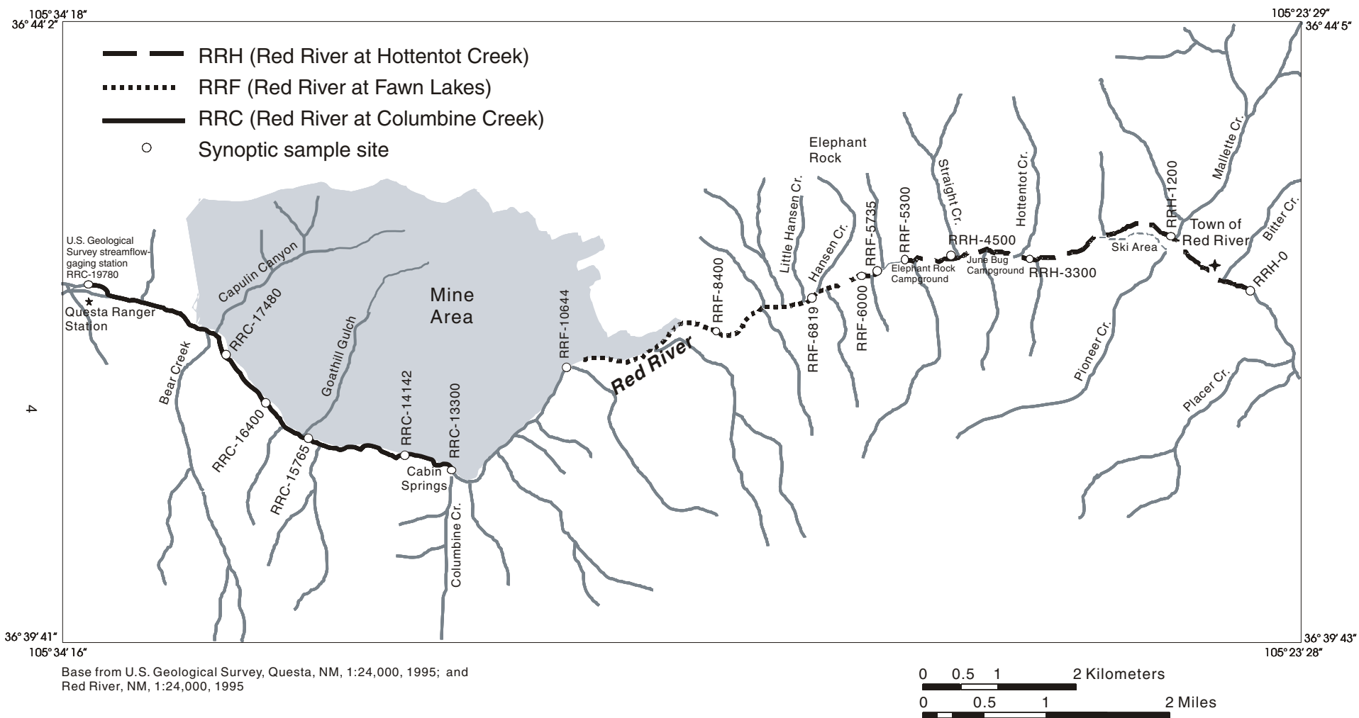
Figure 3. Study reaches and selected synoptic sample sites for the snowmelt tracer study, 2002.
