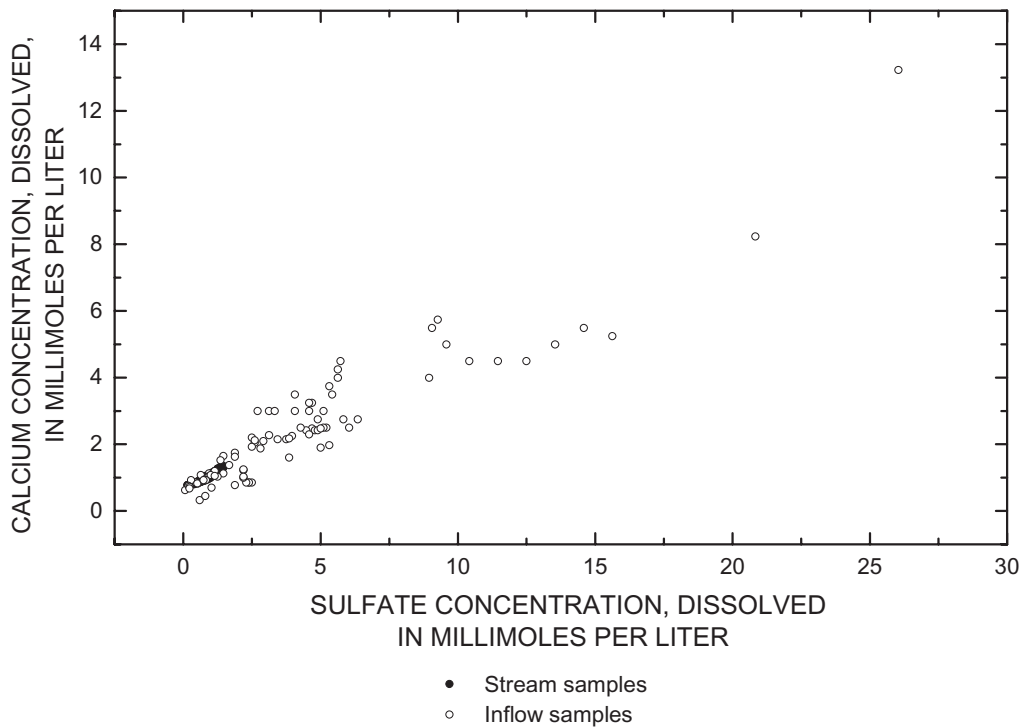
Figure 8. Calcium concentrations in relation to sulfate concentrations.
