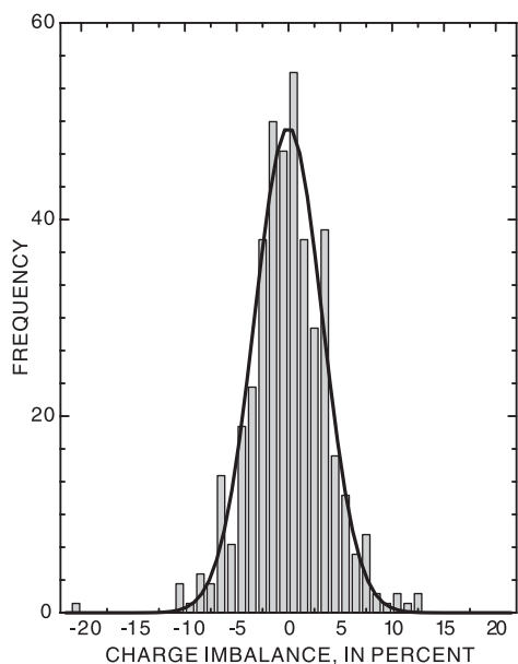
Figure 4. Frequency of charge imbalance for all synoptic samples.
