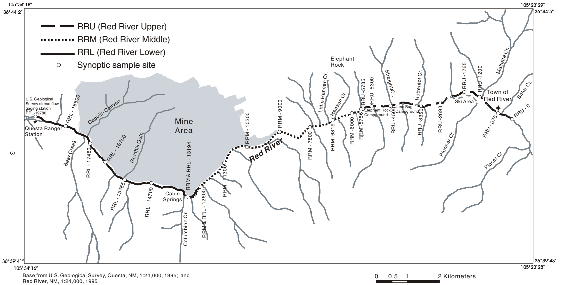
Figure 2. Study reaches and selected synoptic sample sites for the low-flow tracer study, 2001.
