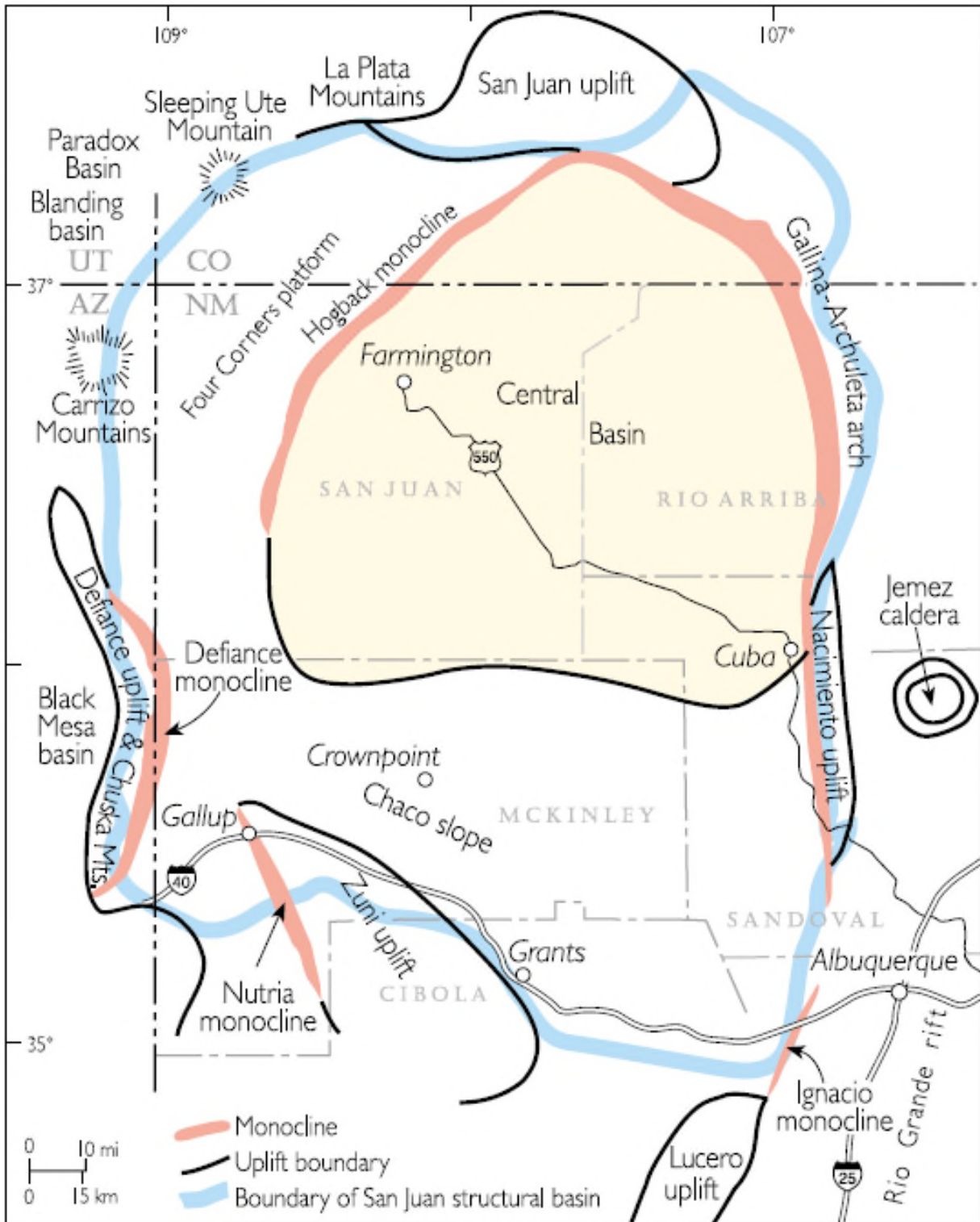
PEABODY EXHIBIT 15. Structural Elements of the San Juan Basin (From Brister and Price, 2002)
