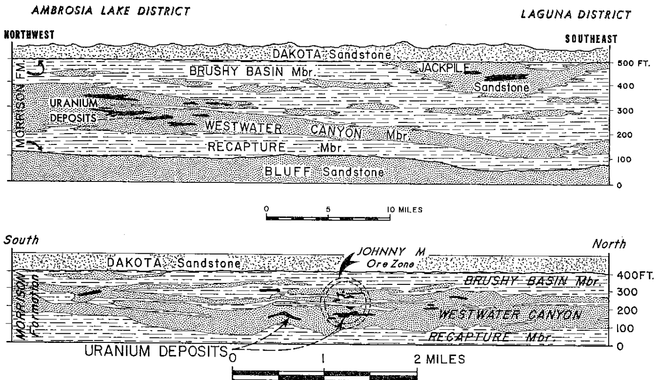
FIGURE 3—GEOLOGIC SECTION SHOWING STRATIGRAPHIC RELATIONS OF THE MORRISON FORMATION. Above: from Ambrosia Lake to Laguna; below: from south to north in Ambrosia Lake district.
