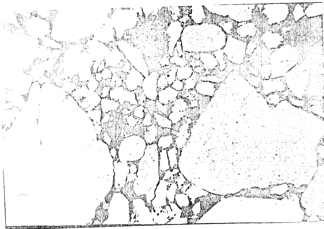
Fig. 20 - Poor sorting in a coarse-grained sandstone (2.5X)
