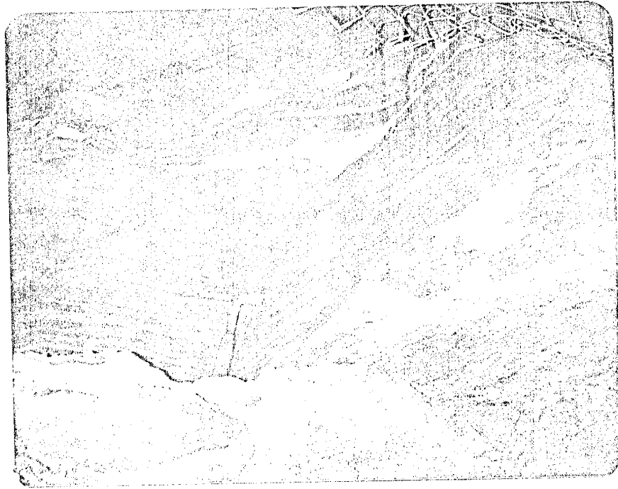
Fig. 22 - Variable color scheme in medium-grained sandstone
