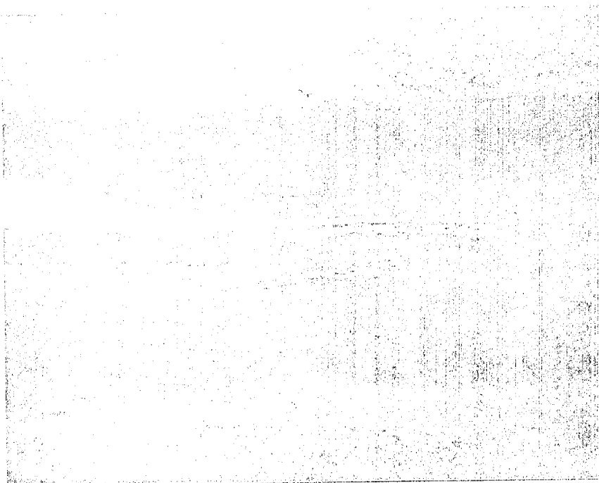
Fig. 40a - Typical Poison Canyon ore
