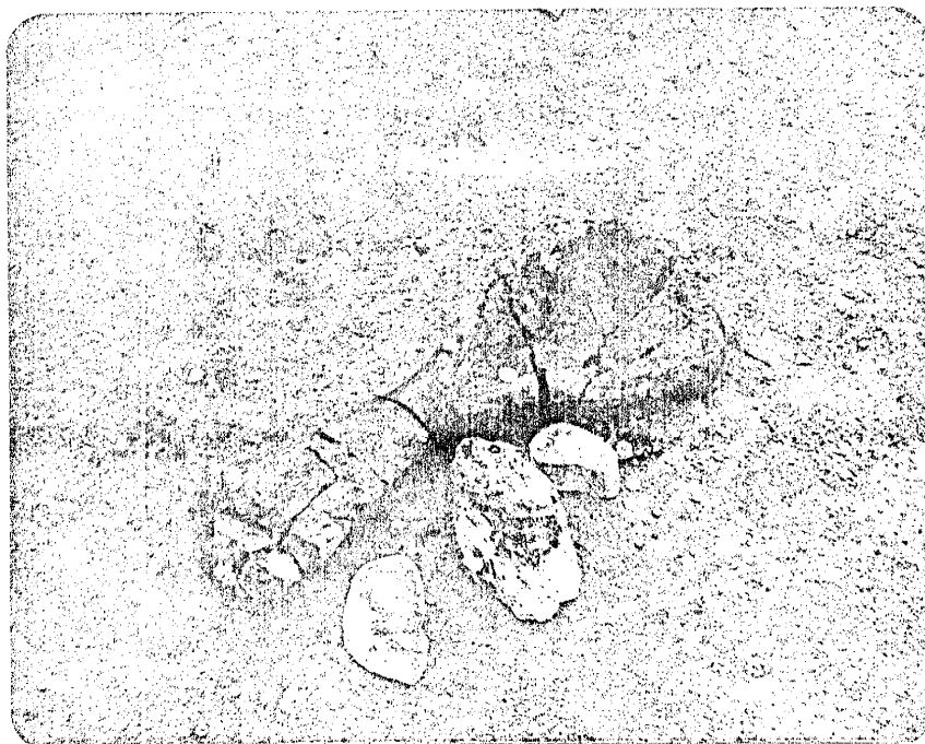
Fig. 24 - Sample of bones collected from the mine; the largest bone in the picture is a reconstruction of several small pieces
