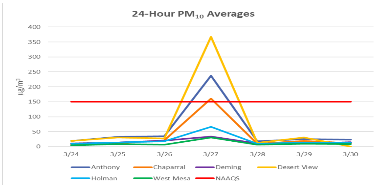
Figure 3-17. 24-Hour PM 10 averages recorded at NMED monitoring sites for the event day and three days before and after.
