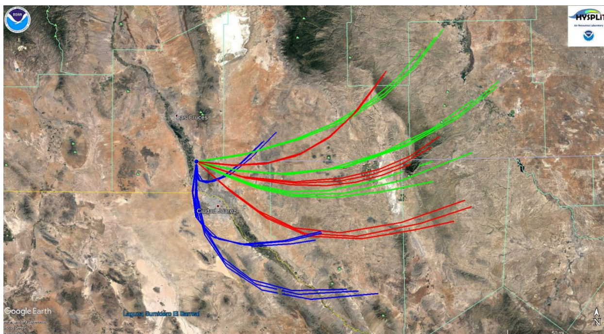
Figure 5-4. HYSPLIT back-trajectory analyses using the Ensemble mode for the Anthony monitoring site
