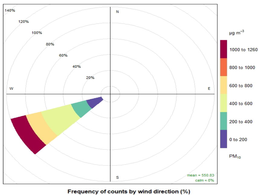
Figure 4-5. Pollution rose for the Chaparral monitoring site
