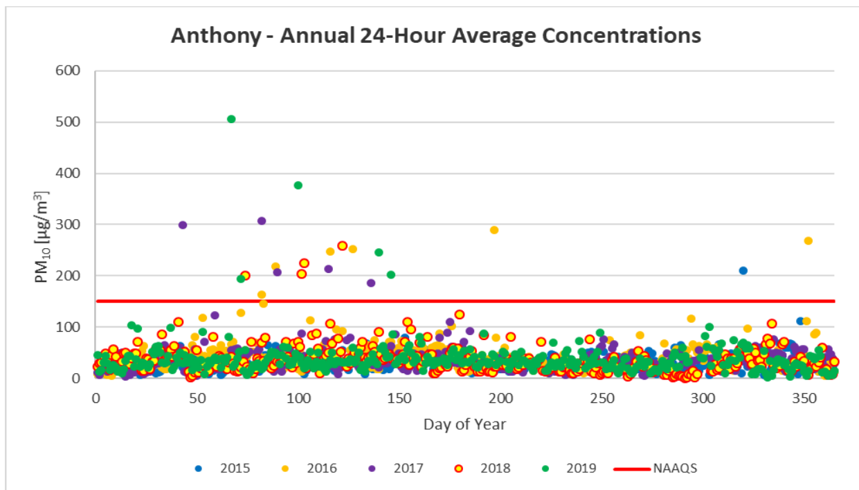
Figure 8-14. 24-hour averages by day of year from 2015-2019 for the Anthony monitoring site.
