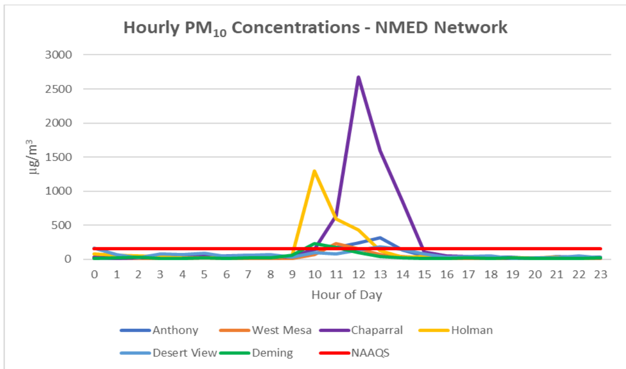
Figure 10-7. NMED monitoring network hourly PM 10 data for the high wind blowing dust event.
