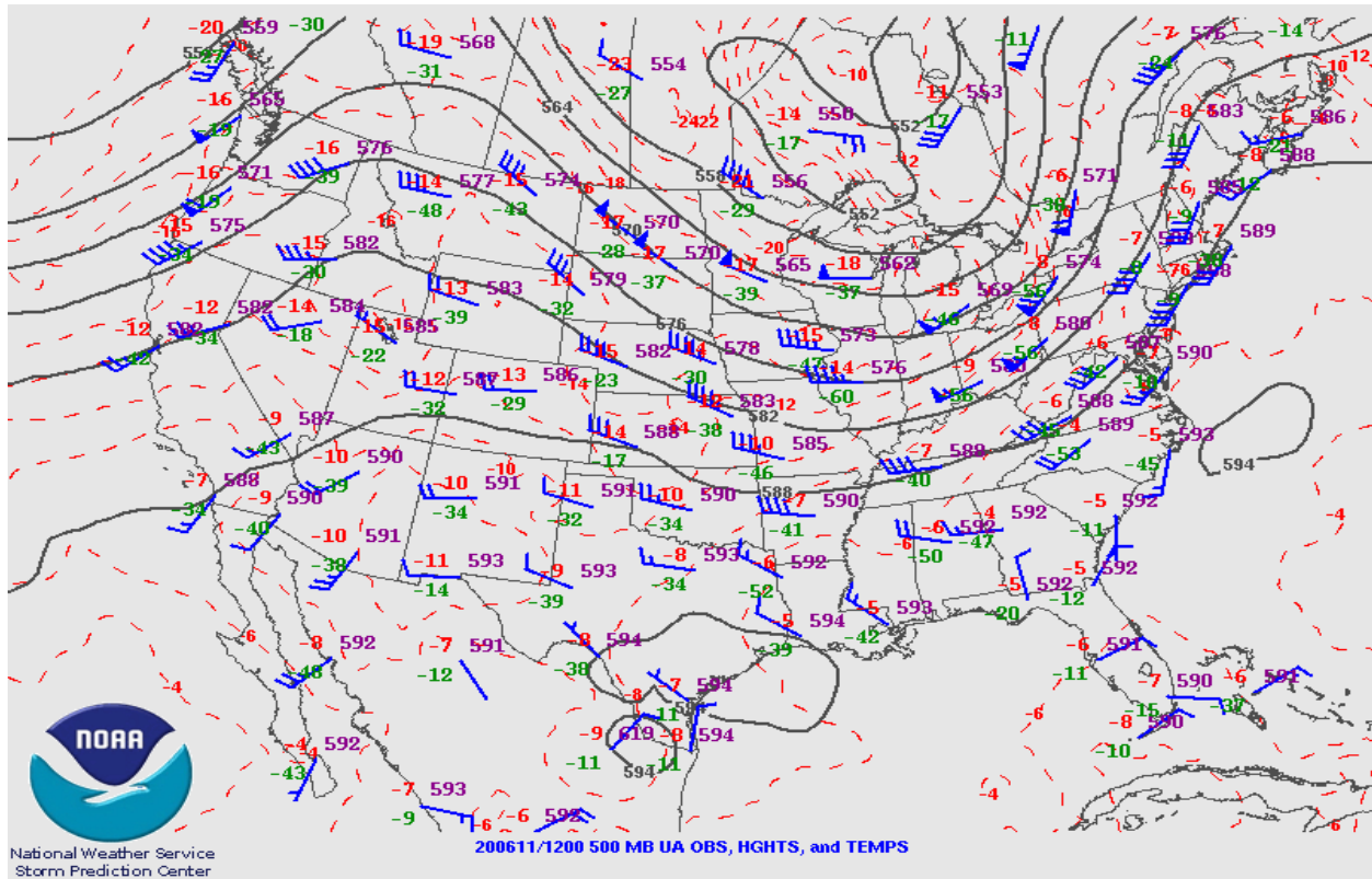
Figure 6-2. Upper air weather map for June 11, 2020 at the 1200 hour. Wind barbs depict wind speed (knots) and direction.
