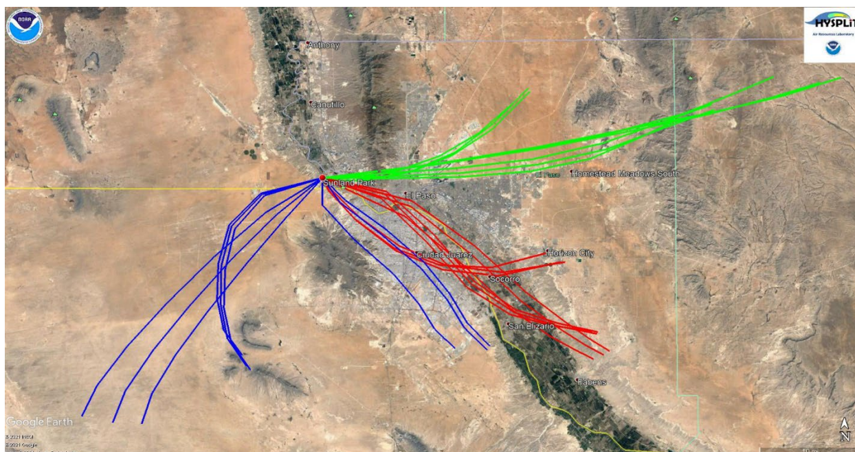
Figure 7-6. HYSPLIT back-trajectory analyses using the Ensemble mode for the Desert View monitoring site.
