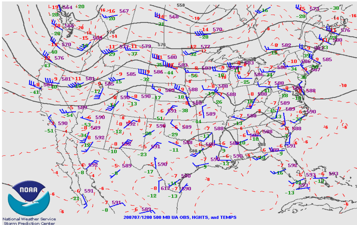
Figure 7-2. Upper air weather map for July 7, 2020 at the 1200 hour. Wind barbs depict wind speed (knots) and direction.
