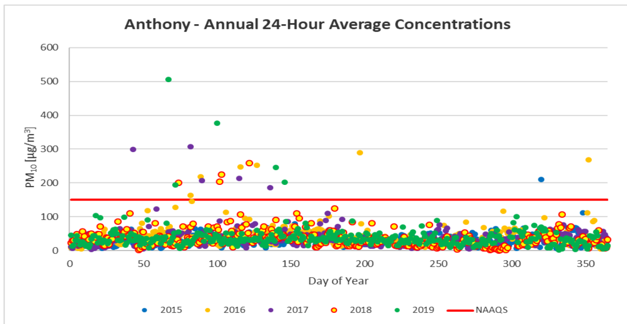
Figure 6-12. 24-hour averages by day of year from 2015-2019 for the Anthony monitoring site.
