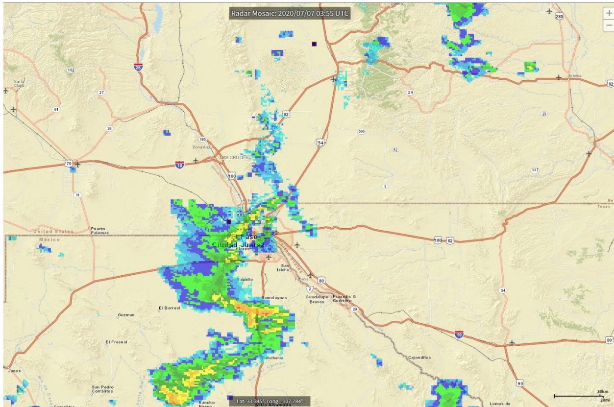
Figure - 12-14. Strong storm cell developed over the Desert View monitoring site extending into northern Chihuahua, Mexico July 6, 2020 at 20:55 (MST). Radar image courtesy of https://www.ncei.noaa.gov/maps/radar/ .
