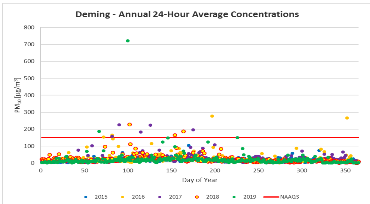
Figure 6-13. 24-hour averages by day of year from 2015-2019 for the Deming monitoring site.
