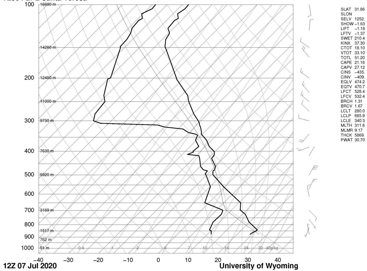
Figure 12-11. NWS Sounding at 05:00 (MST) July 7, 2020 released from Santa Teresa, NM. Note lower wind columns predominating from southeast direction with a temperature inversion. Provided by University of Wyoming.
