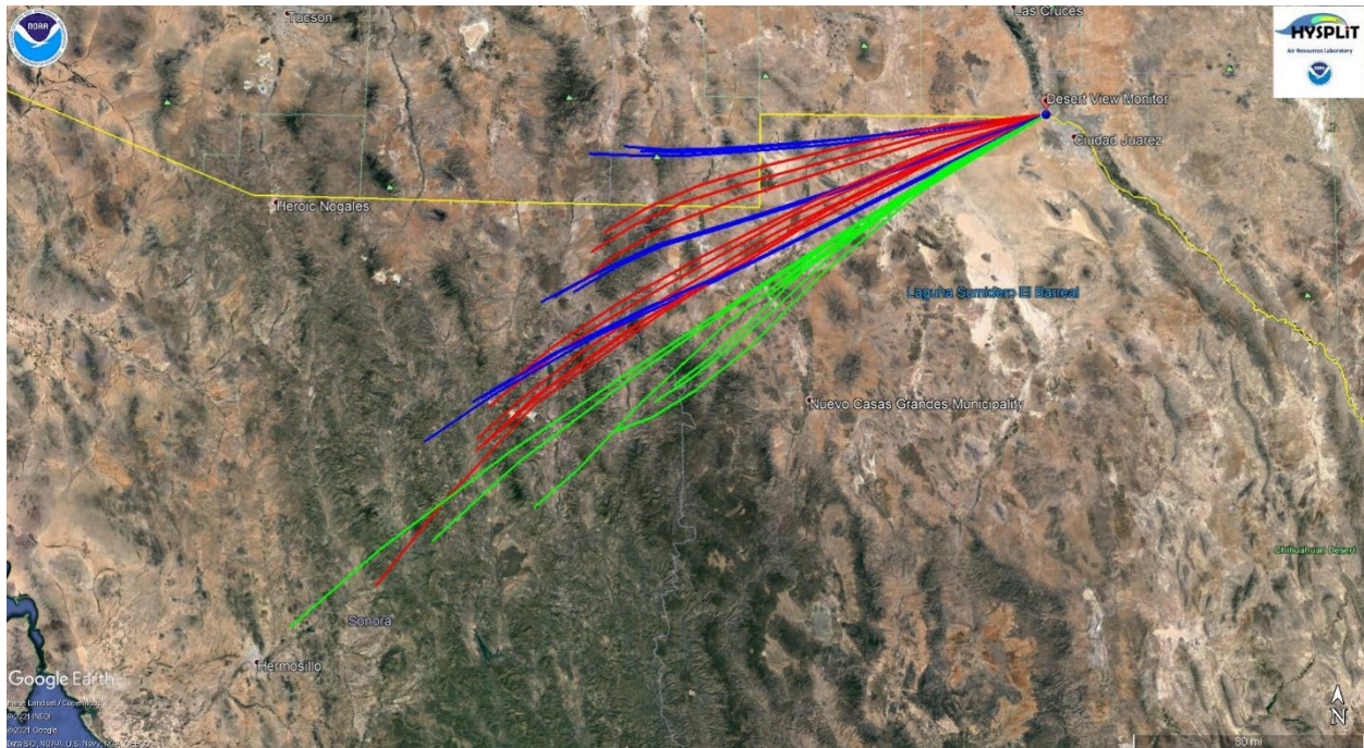
Figure 3-6. HYSPLIT back-trajectory analyses using the Ensemble mode for Desert View monitoring site
