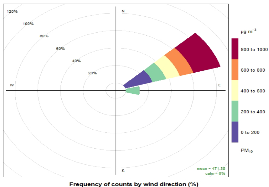
Figure 5-5. Pollution rose for the Anthony monitoring site.
