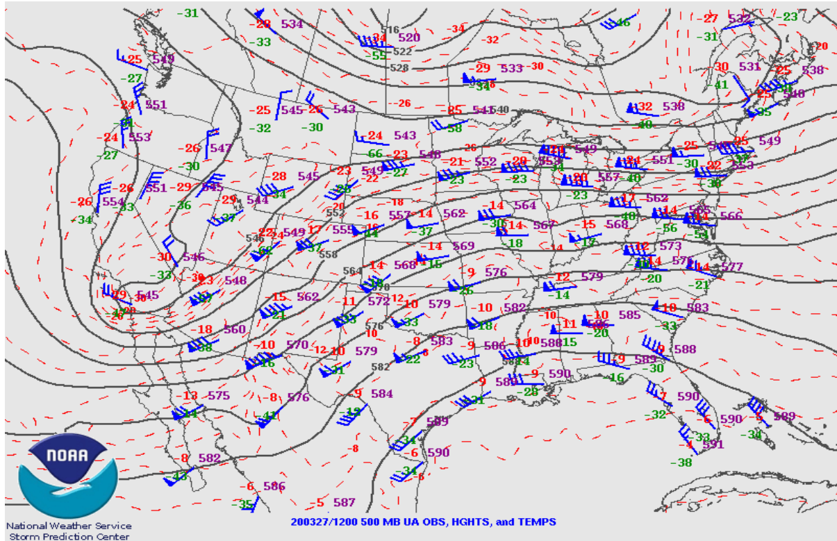
Figure 3-2. Upper air weather map for March 27, 2020 at the 1200 hour. Wind barsbs depict wind speed (knots) and direction.
