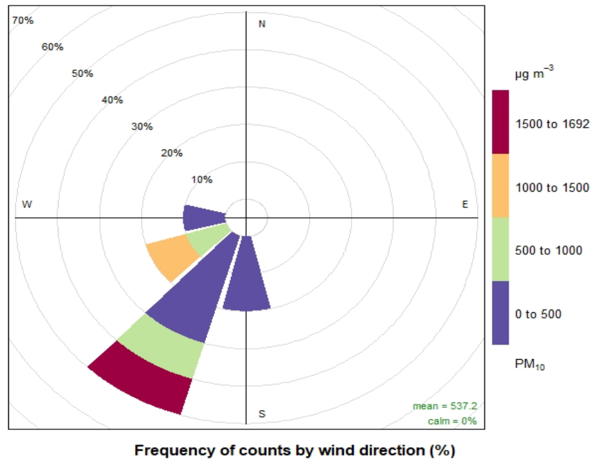
Figure 3-7. Pollution rose for the Anthony monitoring site.
