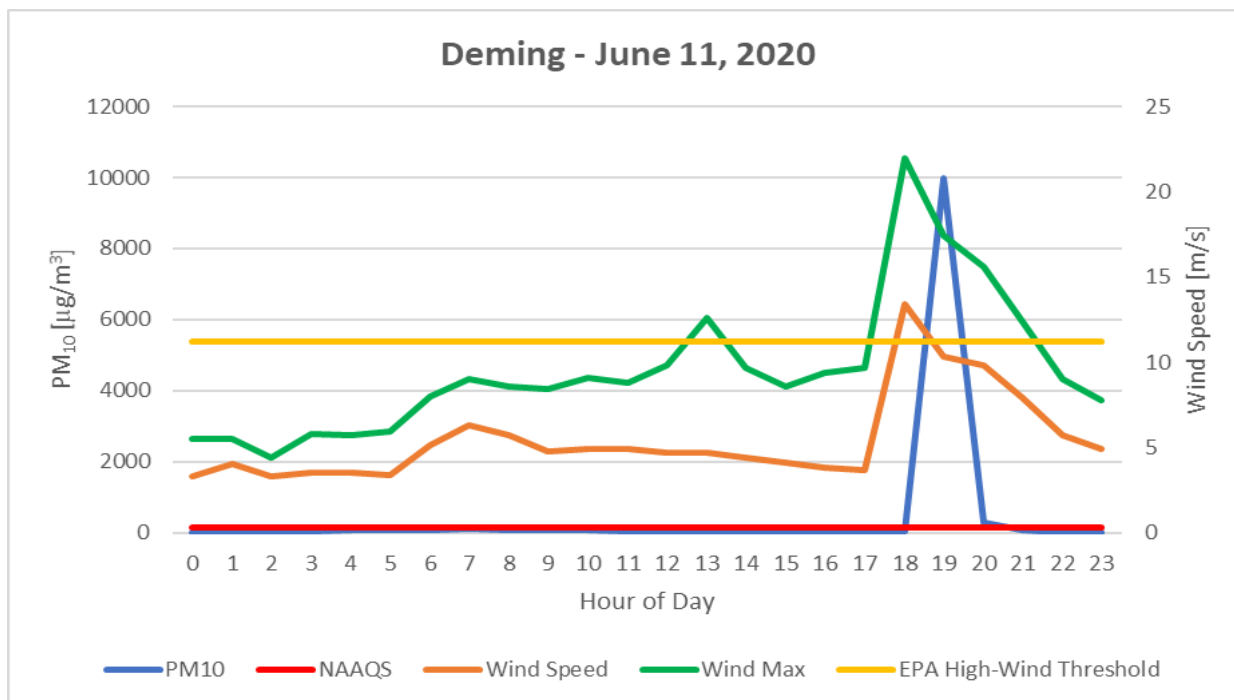
Figure 6-11. Deming monitoring site hourly PM 10 and wind speed data for the high wind blowing dust event.
