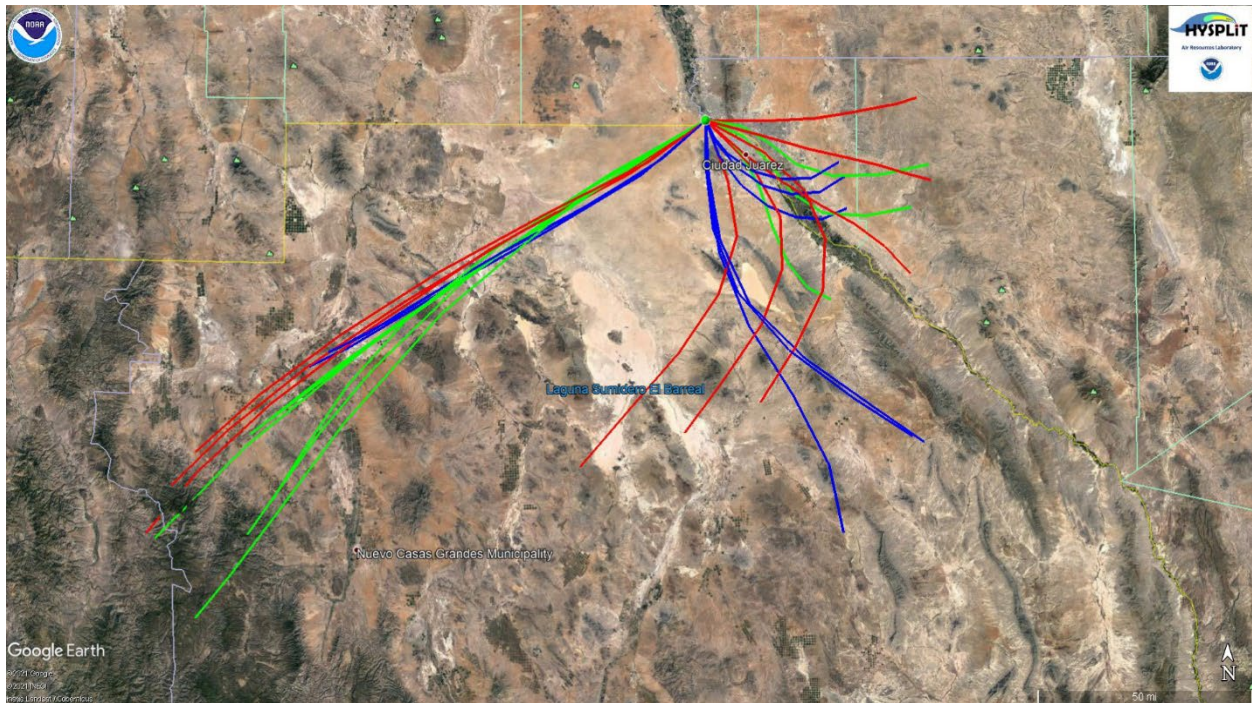
Figure 9-4. HYSPLIT back-trajectory analyses using the Ensemble mode for Desert View monitoring site.
