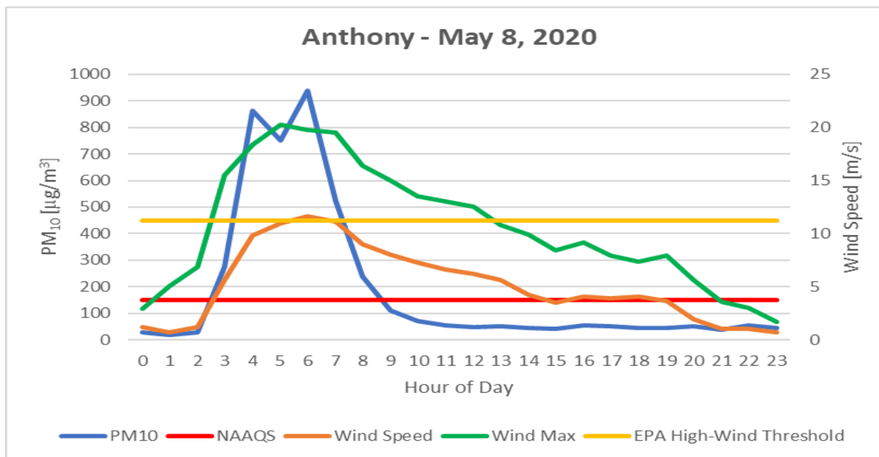
Figure 5-7. Anthony monitoring site hourly PM 10 and wind speed data for the high wind blowing dust event.
