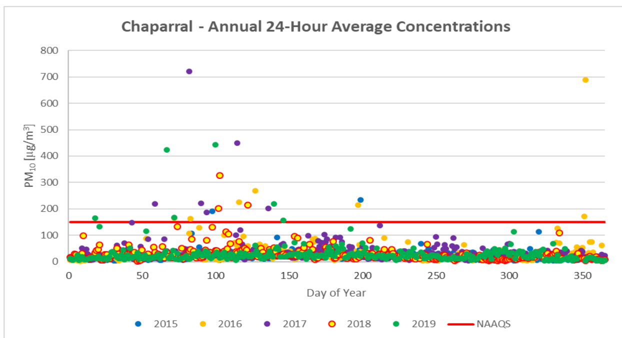
Figure 4-8. 24-hour averages by day of year from 2015-2019.
