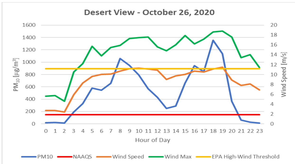
Figure 9-7. Desert View monitoring site hourly PM 10 and wind speed data for the high wind blowing dust event.
