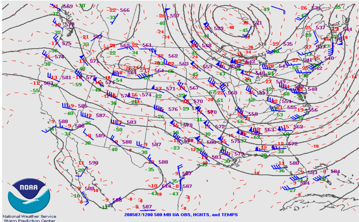
Figure 4-2. Upper air weather map for May 7, 2020 at the 1200 hour. Wind barbs depict wind speed (knots) and direction.
