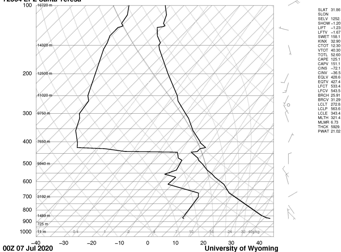
Figure 12-10. NWS Sounding at 17:00 (MST) July 6, 2020 released from Santa Teresa, NM. Provided by University of Wyoming.
