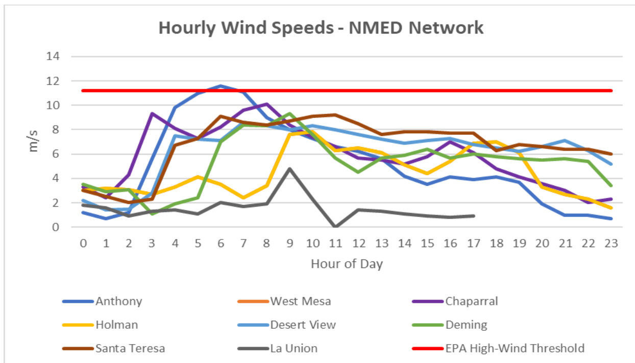
Figure 5-3. Wind speeds at NMED monitoring sites in Doña Ana and Luna Counties.
