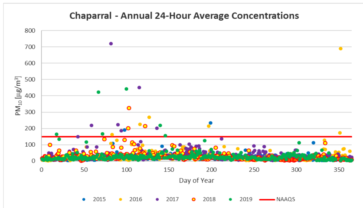
Figure 10-9. 24-hour averages by day of year from 2015-2019 for the Chaparral monitoring site.
