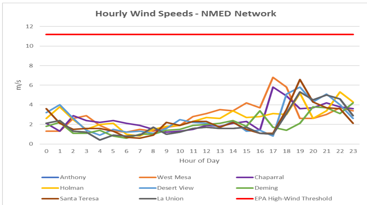
Figure 7-3. Wind speeds at NMED monitoring sites in Doña Ana and Luna Counties.
