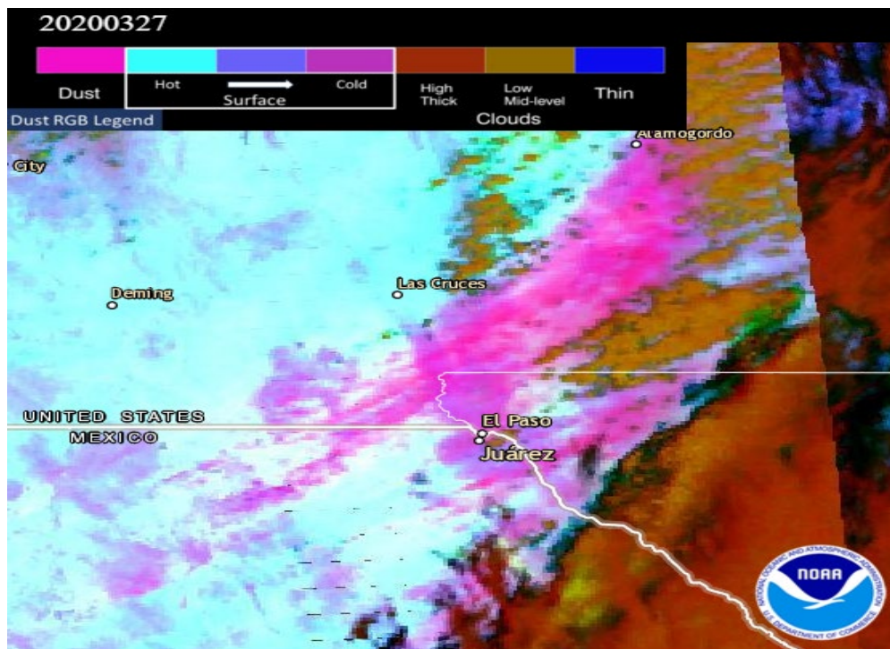
Figure 3-5. VIIRS Suomi NPP satellite dust RGB product imagery showing southwestern New Mexico, northern Chihuahua and western Texas. Imagery obtained from NOAA AerosolWatch website. Note: Pink bands represent dust plumes
