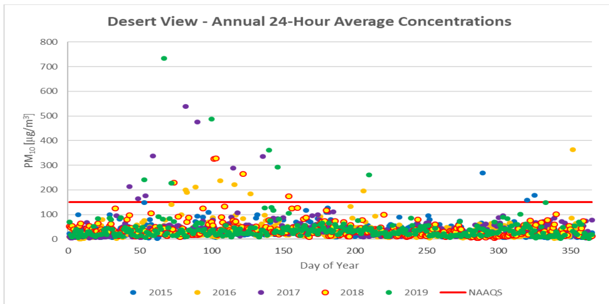
Figure 3-16. 24-hour averages by day of year from 2015-2019 for the Desert View monitoring site.
