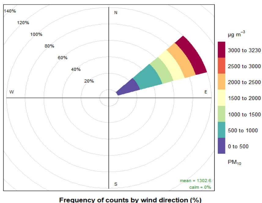
Figure 8-7. Pollution rose for the Anthony monitoring site.
