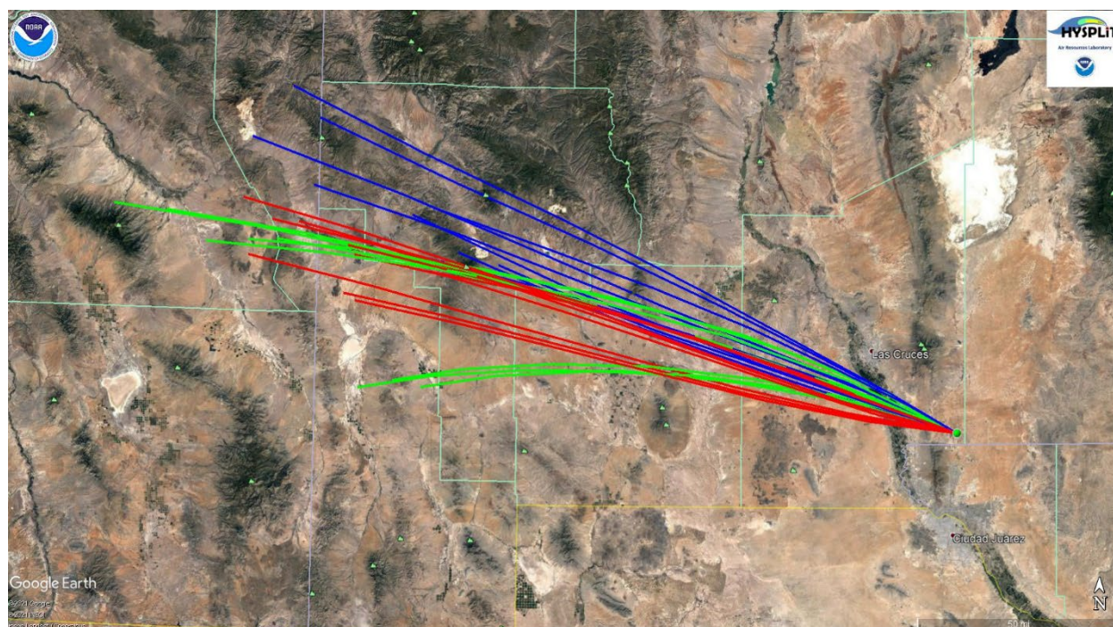
Figure 10-5. HYSPLIT back-trajectory analyses using the Ensemble mode for Chaparral monitoring site.
