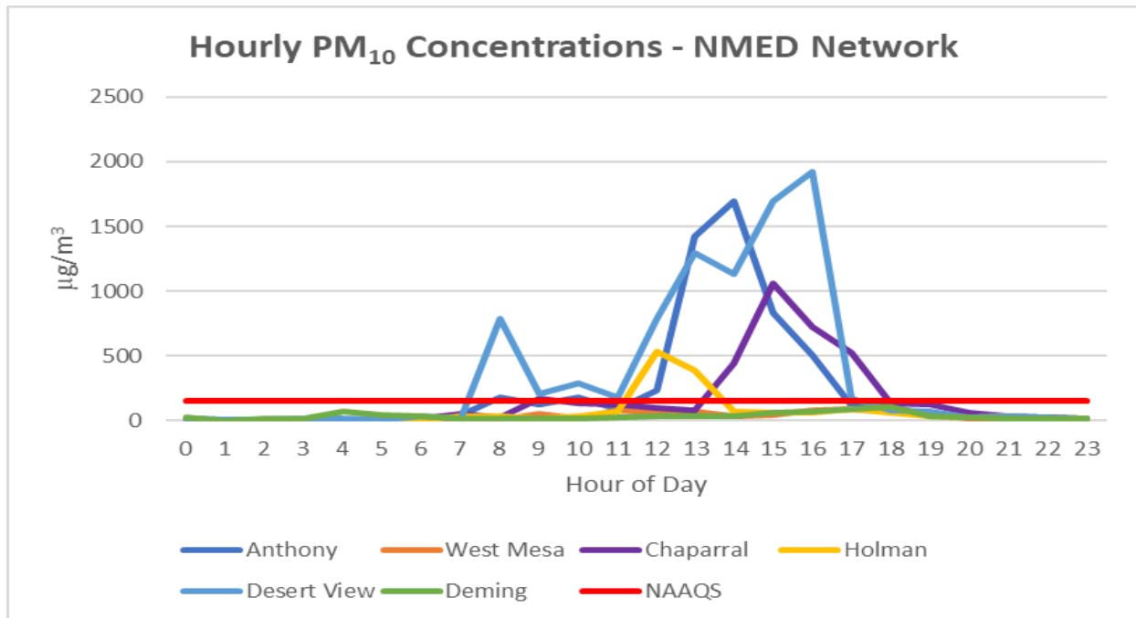
Figure 3-10. NMED monitoring network hourly \text{PM}_{10} data for the high wind blowing dust event.
