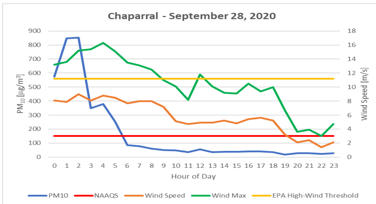
Figure 8-12. Chaparral monitoring site hourly PM 10 and wind speed data for the high wind blowing dust event.
