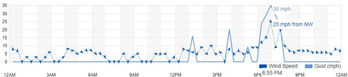
Figure 7-4. Las Cruces Airport 20-minute wind speed data for July 7, 2020. Obtained from WeatherUnderground.com
