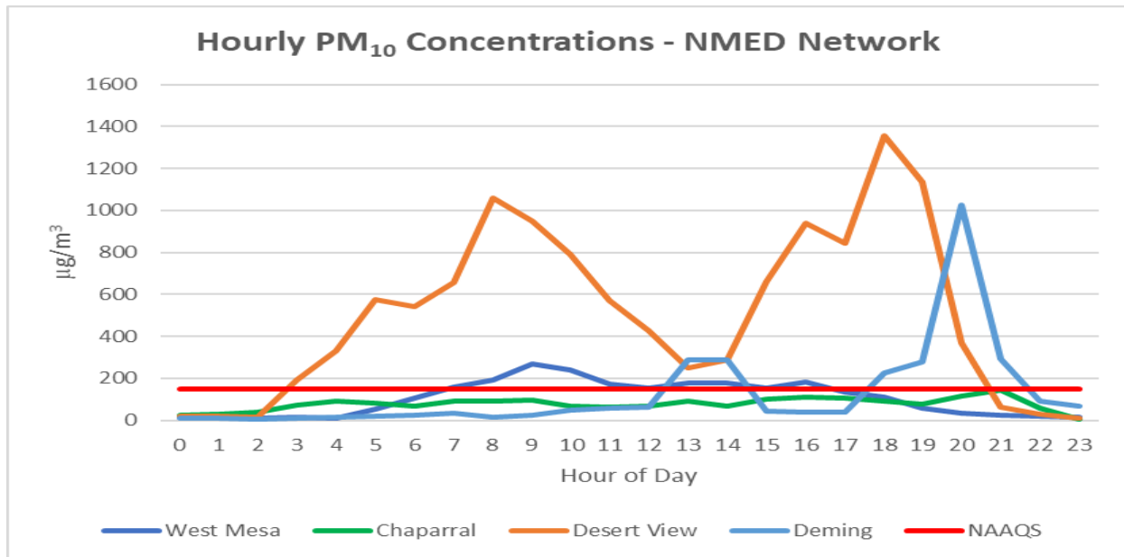
Figure 9-6. NMED monitoring network hourly PM 10 data for the high wind blowing dust event.
