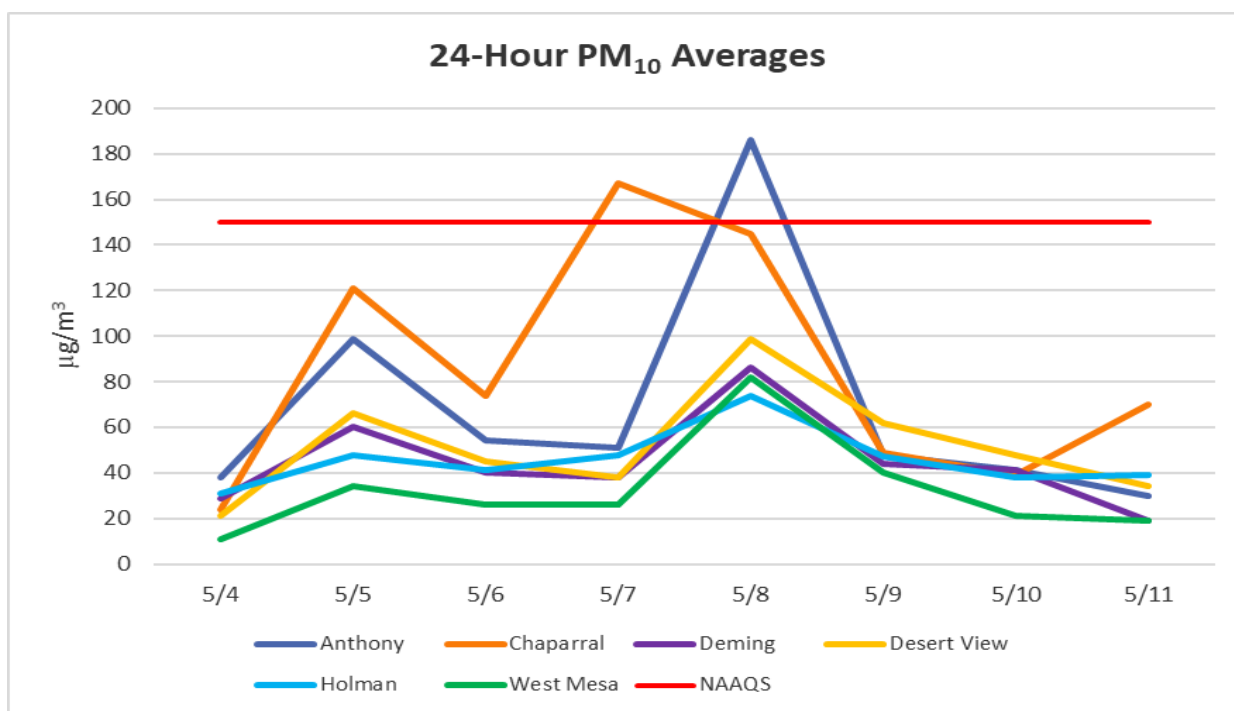
Figure 5-9. 24-Hour PM 10 averages recorded at NMED monitoring sites for the event day and three days before and after.
