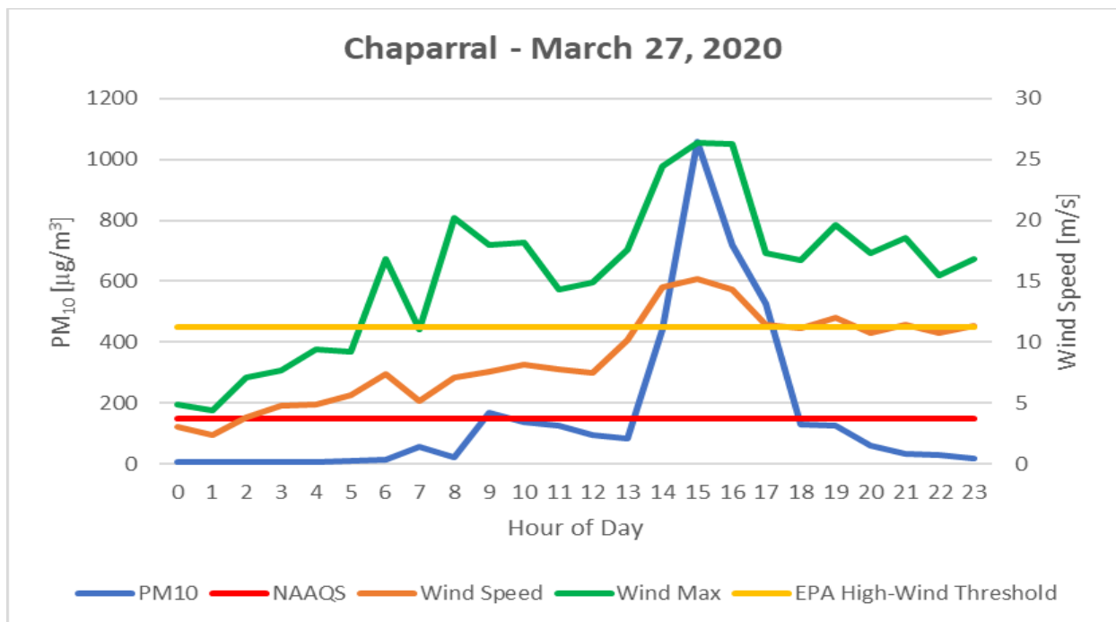
Figure 3-12. Chaparral monitoring site hourly PM 10 and wind speed data for the high wind blowing dust event.
