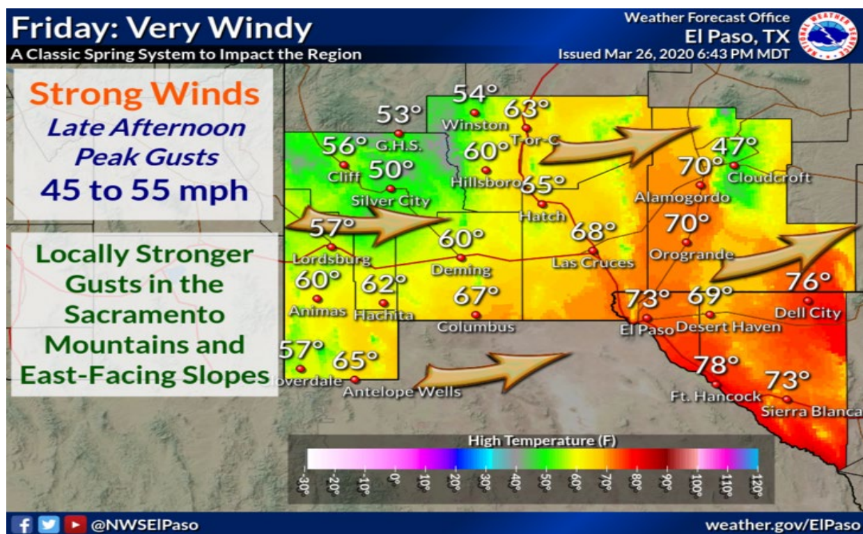
Figure 3-3. KTSM Forecast Graphic for the event.
