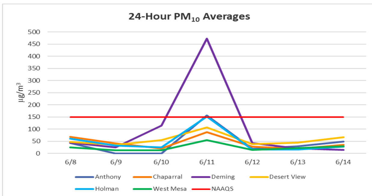
Figure 6-14. 24-Hour PM 10 averages recorded at NMED monitoring sites for the event day and three days before and after.
