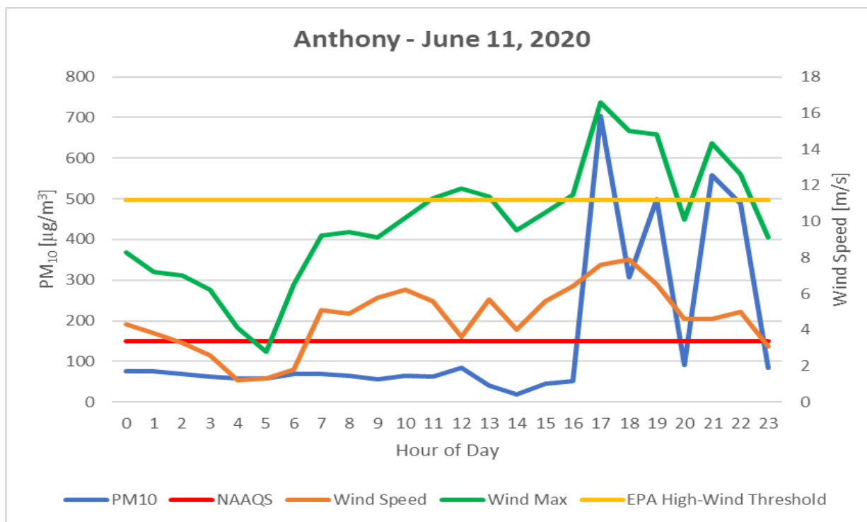
Figure 6-10. Anthony monitoring site hourly PM 10 and wind speed data for the high wind blowing dust event.
