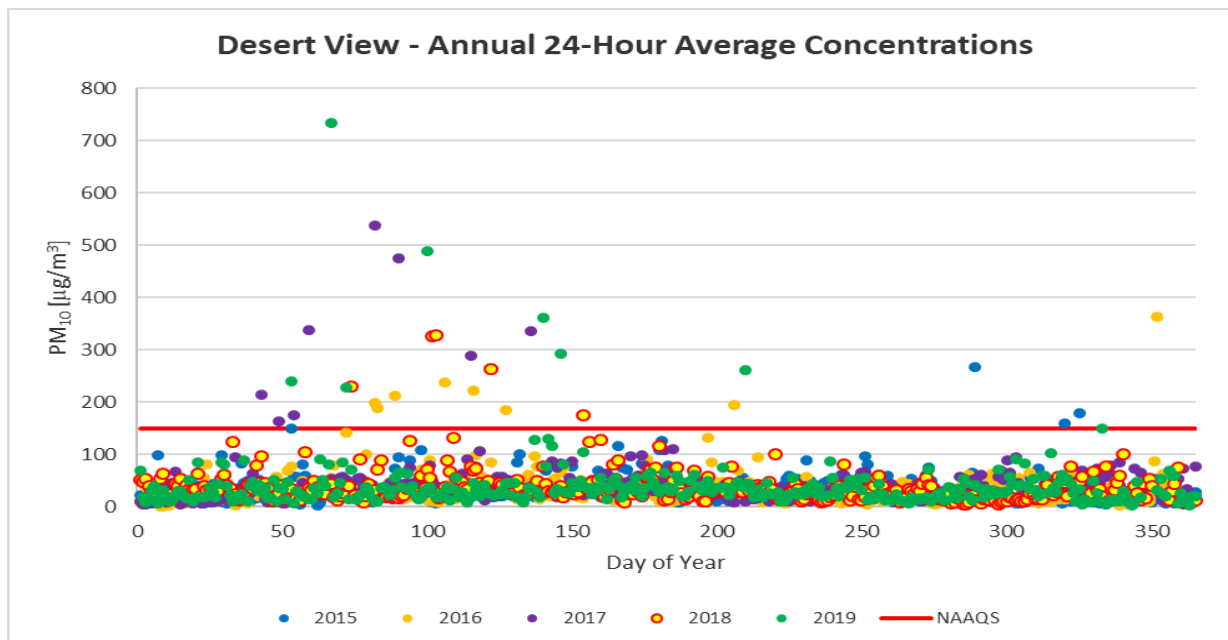
Figure 9-8. 24-hour averages by day of year from 2015-2019 for the Desert View monitoring site.
