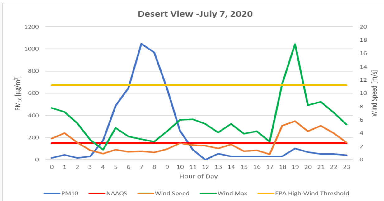
Figure 7-9. Desert View monitoring site hourly PM 10 and wind speed data for the high wind blowing dust event.
