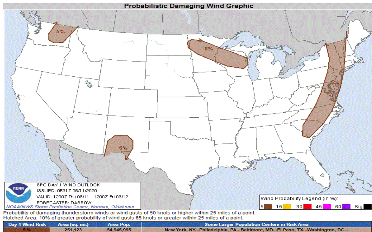
Figure 6-3. NWS Wind forecast product provided for June 11, 2020
