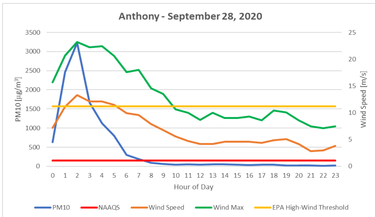
Figure 8-11. Anthony monitoring site hourly PM 10 and wind speed data for the high wind blowing dust event.
