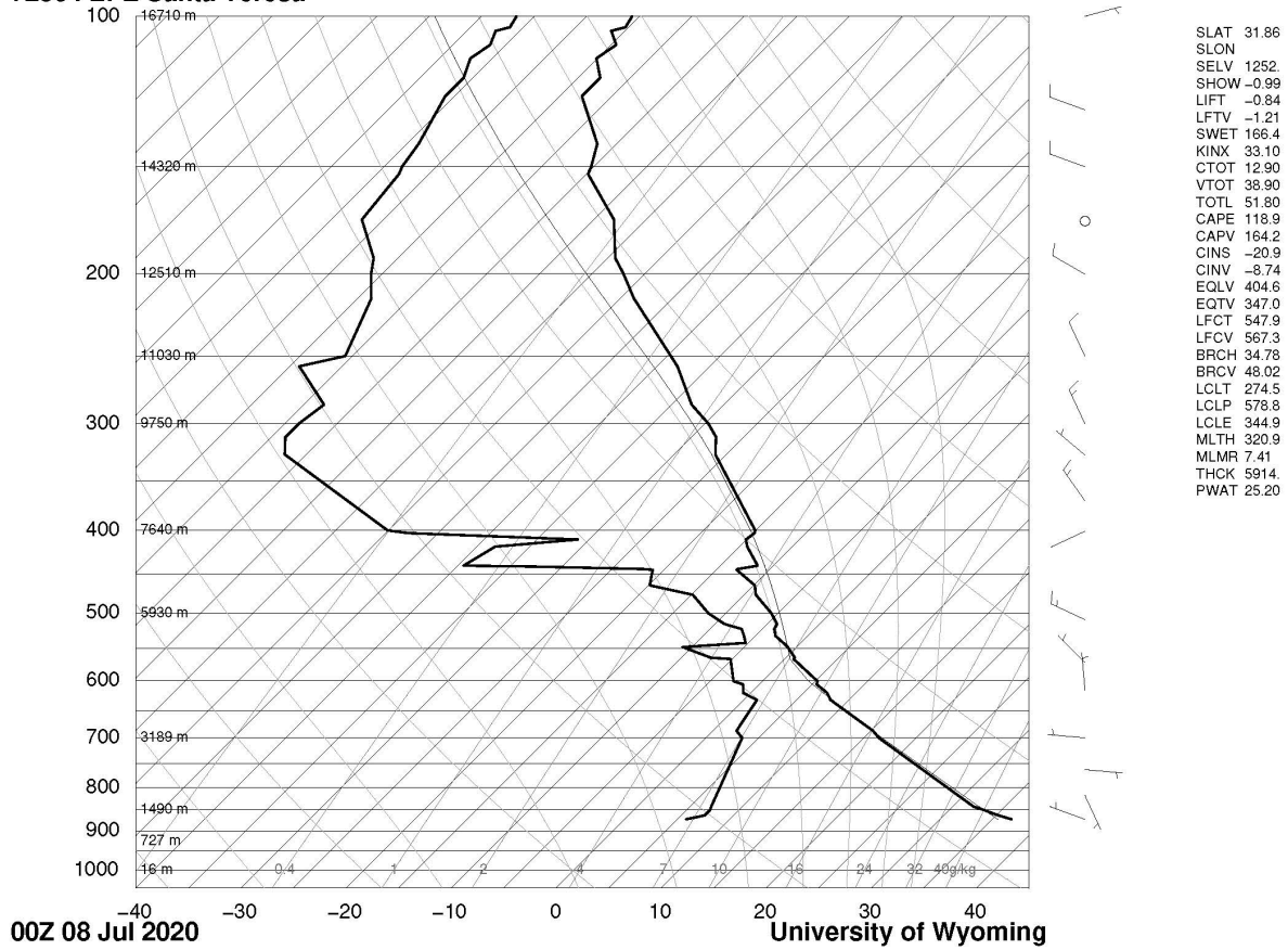
Figure 12-12. NWS Sounding at 17:00 (MST) July 7, 2020 released from Santa Teresa, NM. Provided by University of Wyoming.
