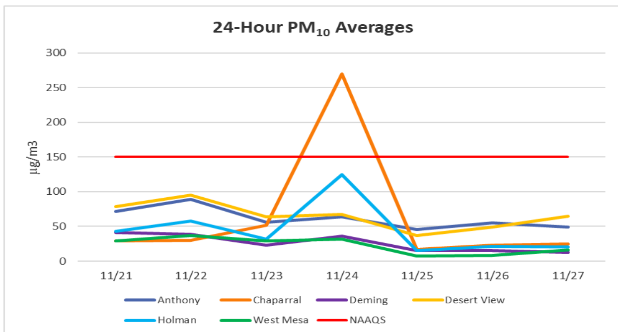
Figure 10-10. 24-Hour PM 10 averages recorded at NMED monitoring sites for the event day and three days before and after.
