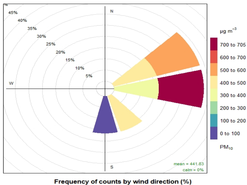
Figure 6-7. Pollution rose for the Anthony monitoring site.
