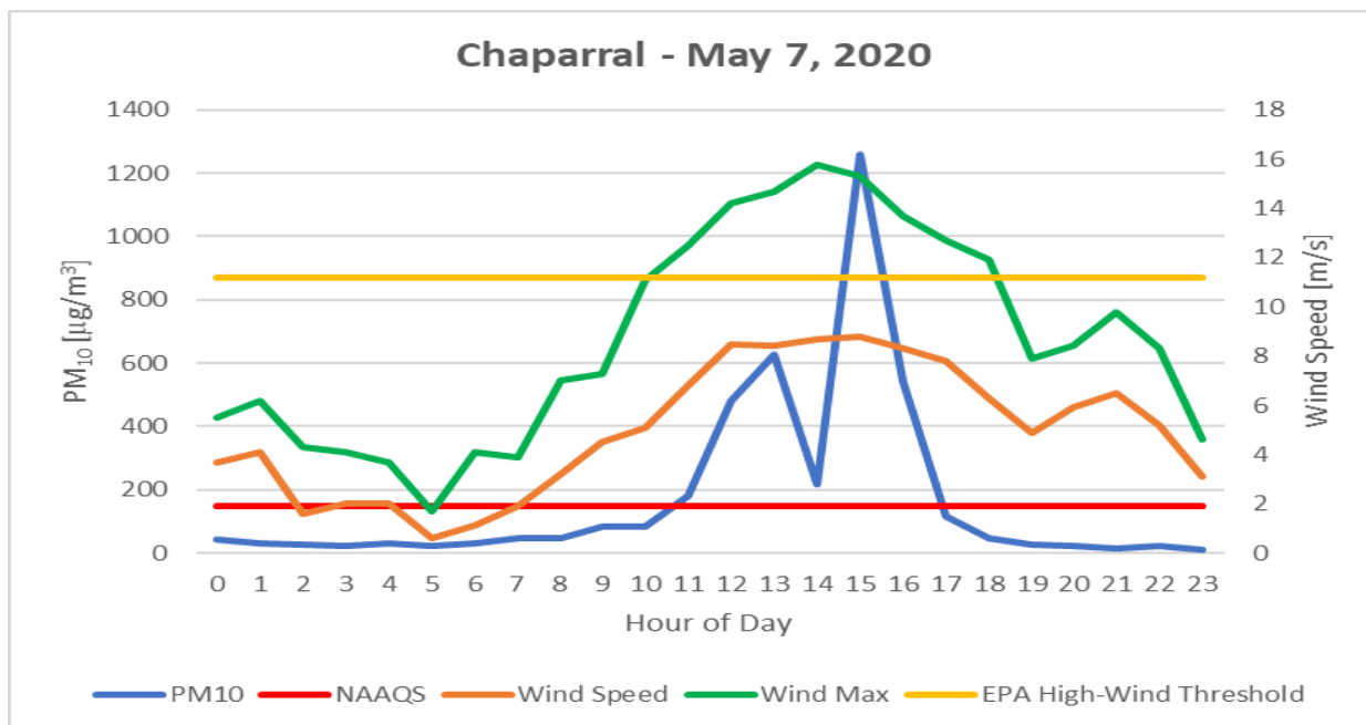
Figure 4-7. Chaparral monitoring site hourly PM 10 and wind speed data for the high wind blowing dust event.
