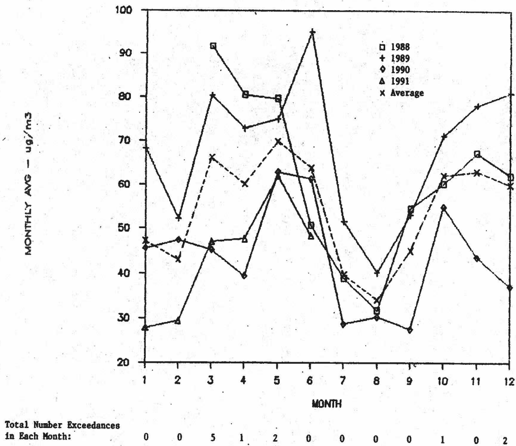
Figure 3 PM-10 MONTHLY AVERAGES – ANTHONY, NM
