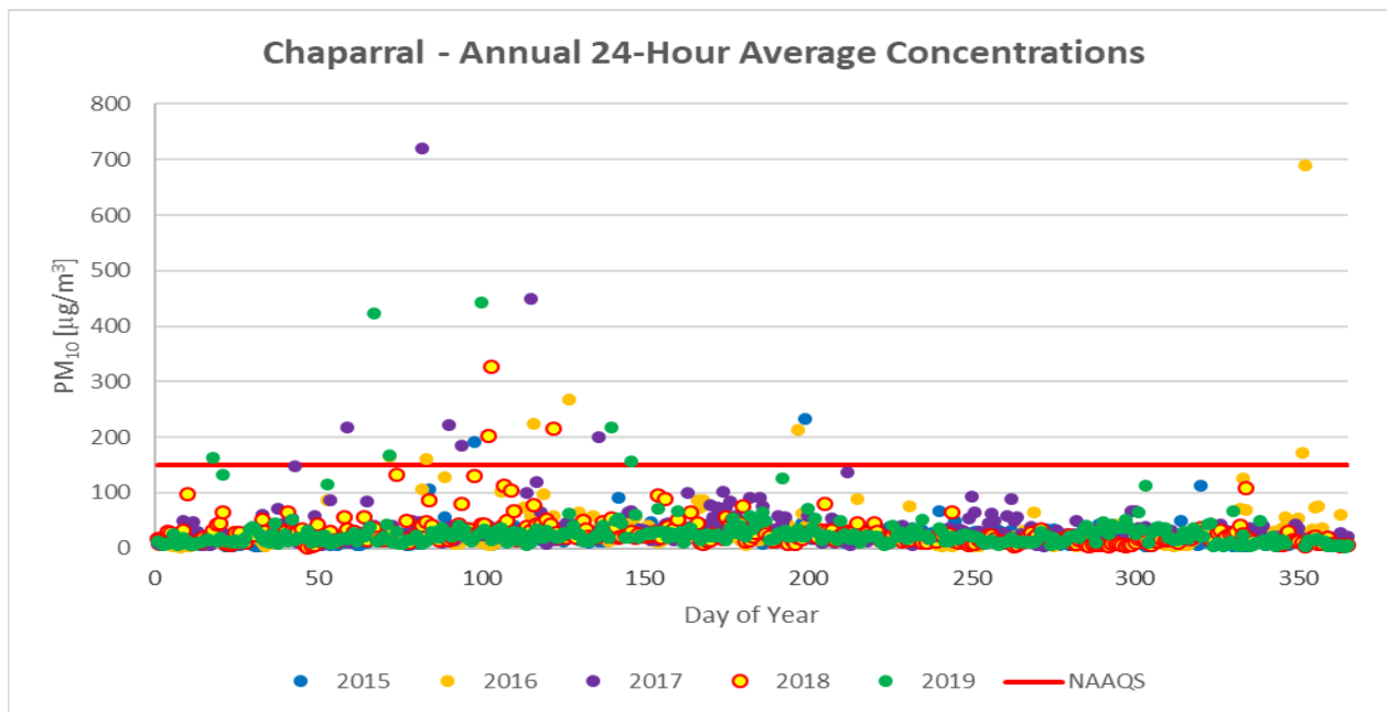
Figure 3-15. 24-hour averages by day of year from 2015-2019 for the Chaparral monitoring site.
