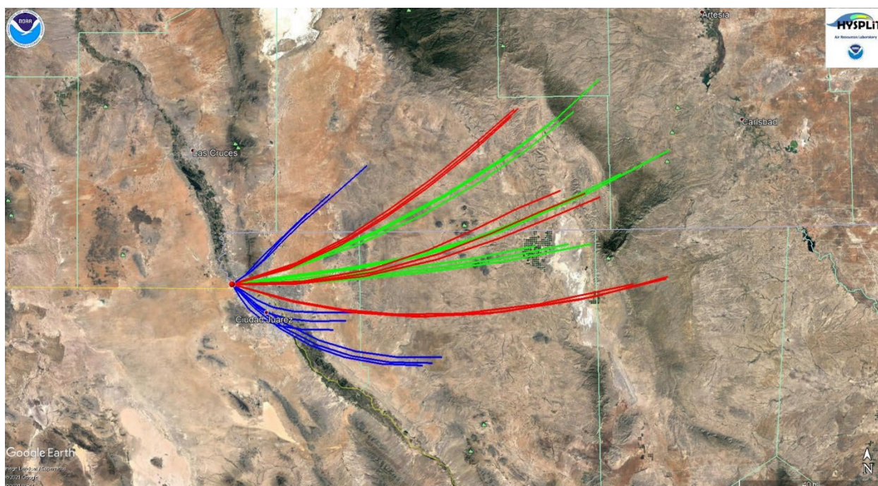
Figure 8-6. HYSPLIT back-trajectory analyses using the Ensemble mode for the Desert View monitoring site.
