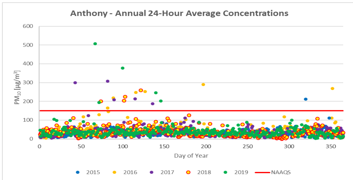
Figure 3-14. 24-Hour averages by day of year from 2015-2019 for the Anthony monitoring site.
