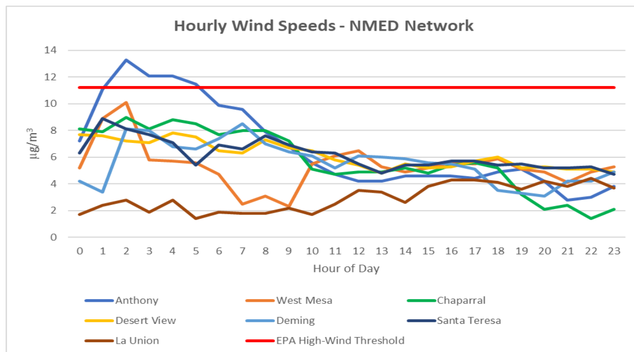
Figure 8-4. Wind speeds at NMED monitoring sites in Doña Ana and Luna Counties.
