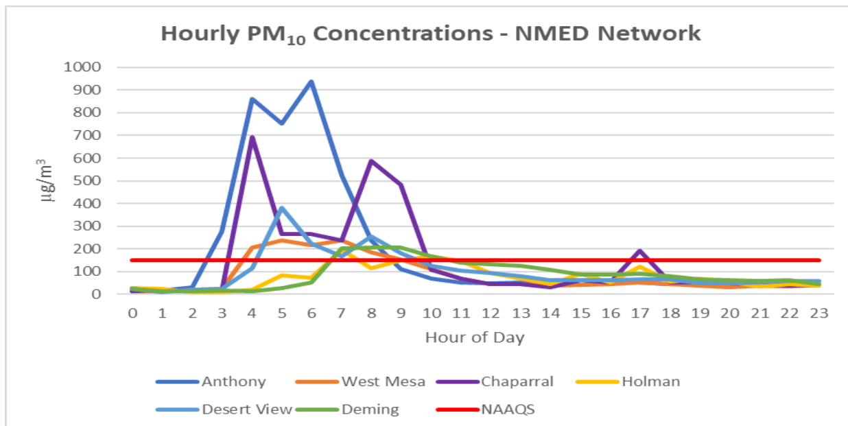
Figure 5-6. NMED monitoring network hourly PM 10 data for the high wind blowing dust event.
