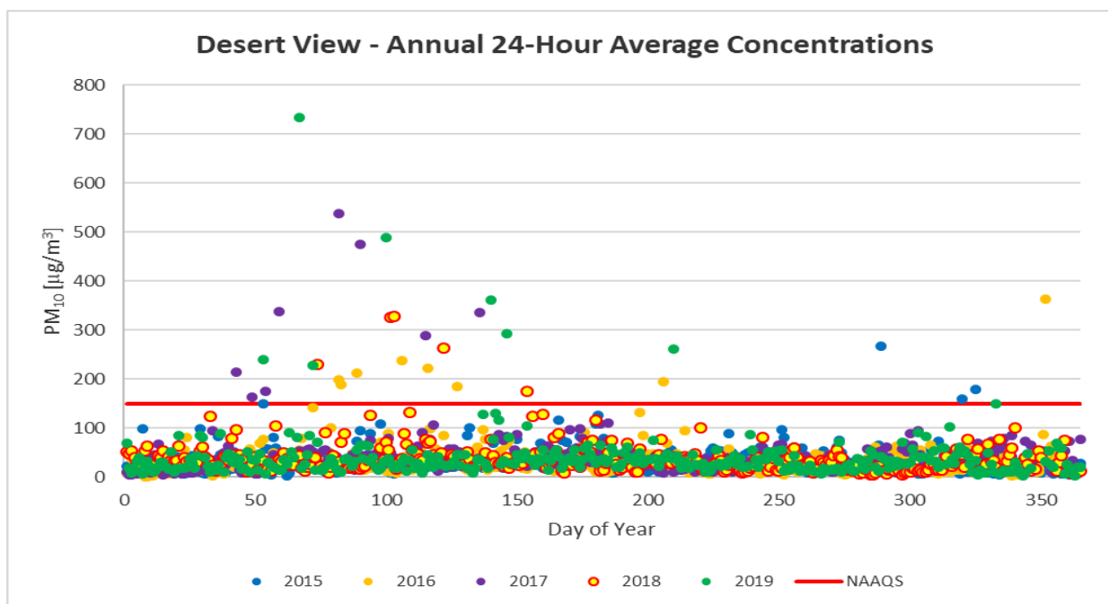
Figure 7-10. 24-hour averages by day of year from 2015-2019 for the Desert View monitoring site.
