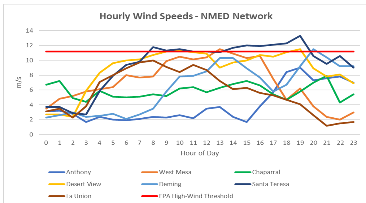
Figure 9-3. Wind speeds at NMED monitoring sites in Doña Ana and Luna Counties.
