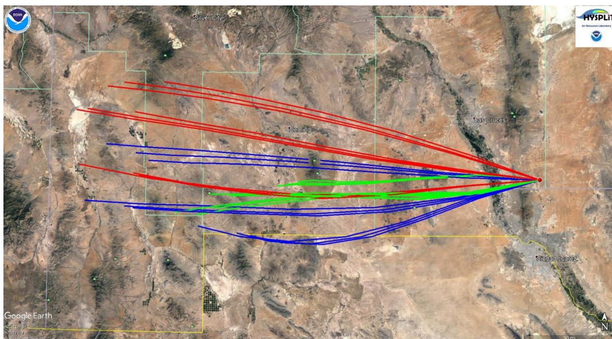
Figure 4-4. HYSPLIT back-trajectory analyses using the Ensemble mode for the Chaparral monitoring site.
