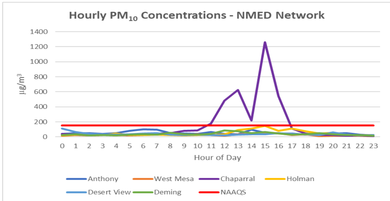
Figure 4-6. NMED monitoring network hourly PM 10 data for the high wind blowing dust event.
