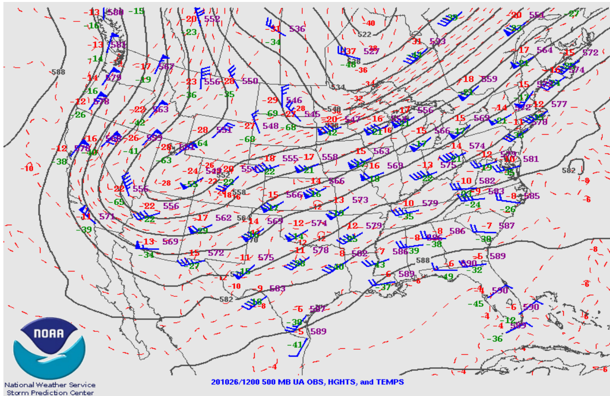
Figure 9-2. Upper air weather map for October 26, 2020 at the 1200 hour. Wind barbs depict wind speed (knots) and direction.
