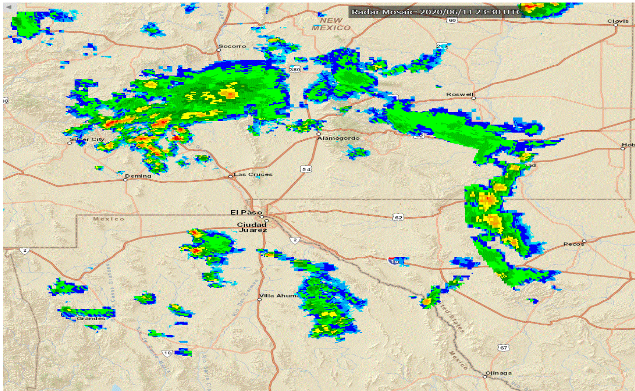
Figure 6-5. NOAA National Reflectivity Radar Mosaic showing southwestern New Mexico, northern Chihuahua and western Texas.
