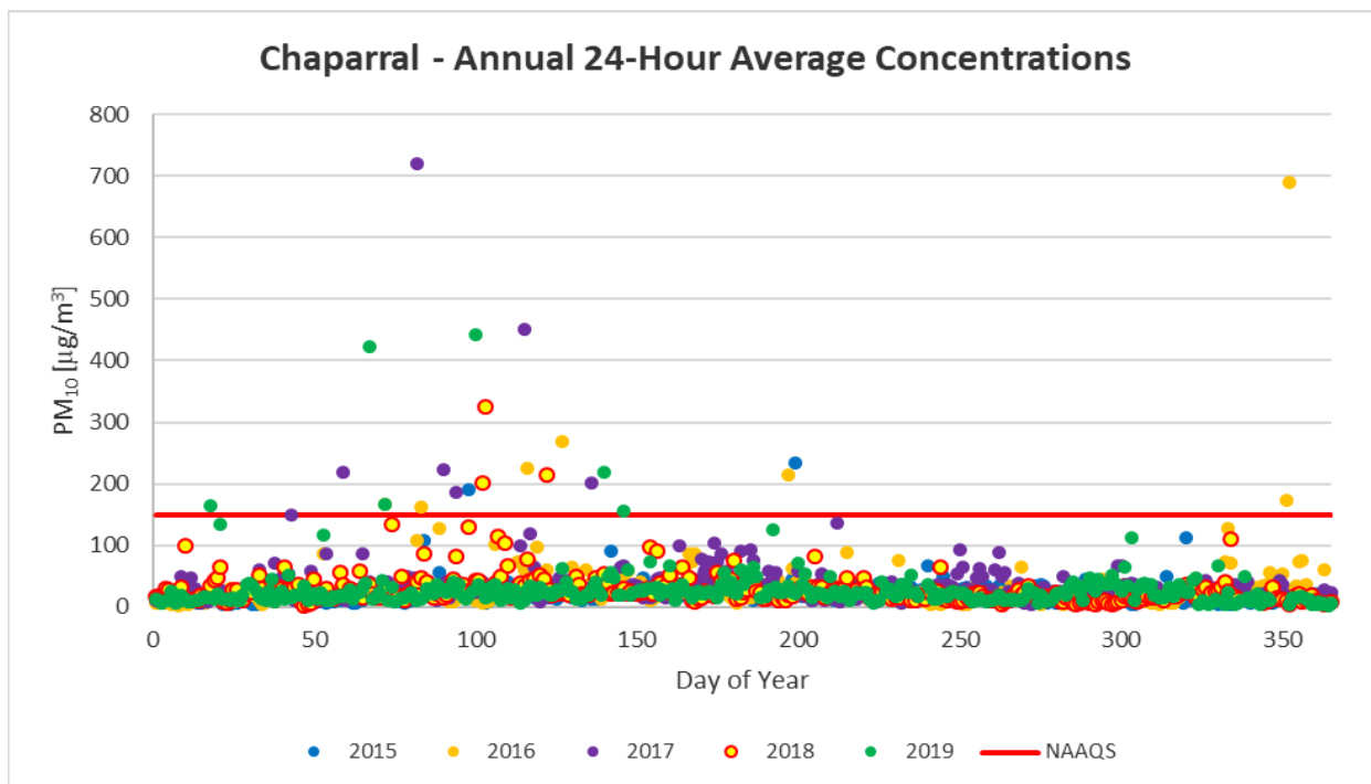
Figure 8-15. 24-hour averages by day of year from 2015-2019 for the Chaparral monitoring site.
