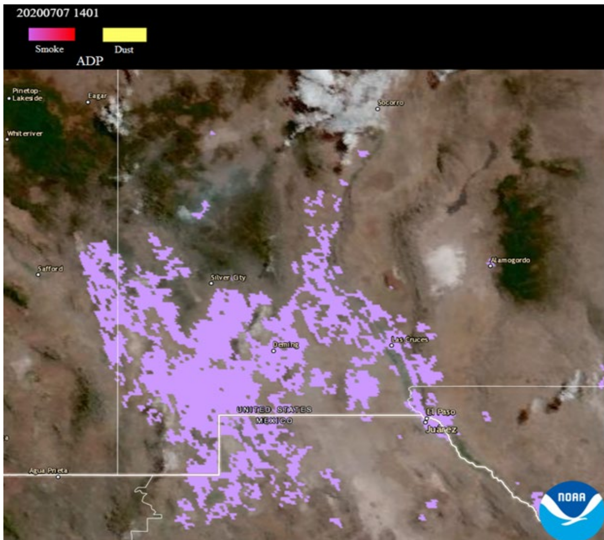
Figure 12-5. GOES-16 Smoke and Dust Mask product showing thick smoke over Desert View Monitoring site July 7, 2020 at 07:01 (MST). Obtained from NOAA AerosolWatch.
