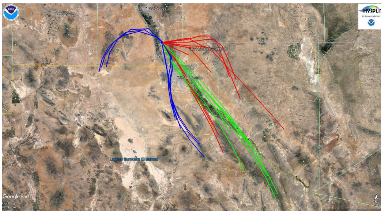
Figure 6-6. HYSPLIT back-trajectory analyses using the Ensemble mode for the Anthony monitoring site.
