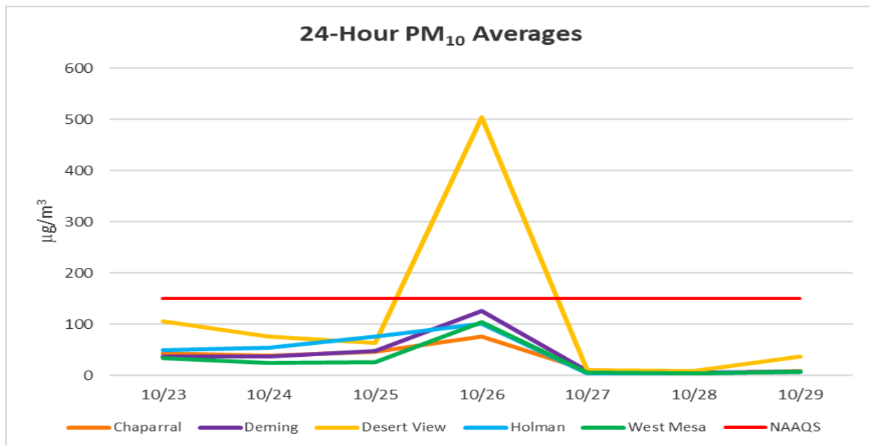
Figure 9-9. 24-Hour PM 10 averages recorded at NMED monitoring sites for the event day and three days before and after.
