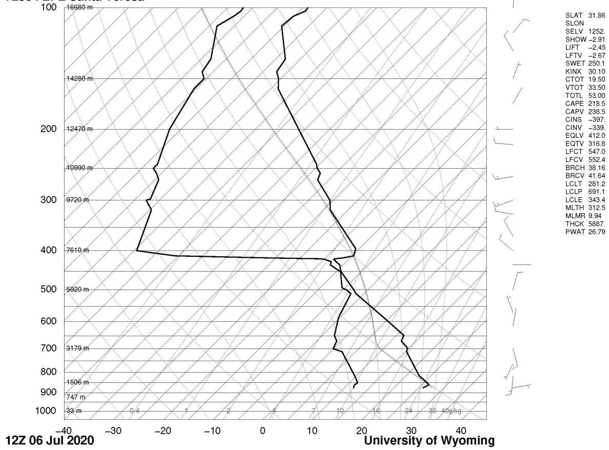
Figure 12-9. NWS Sounding at 05:00 (MST) July 6, 2020 released from Santa Teresa, NM. Provided by University of Wyoming.
