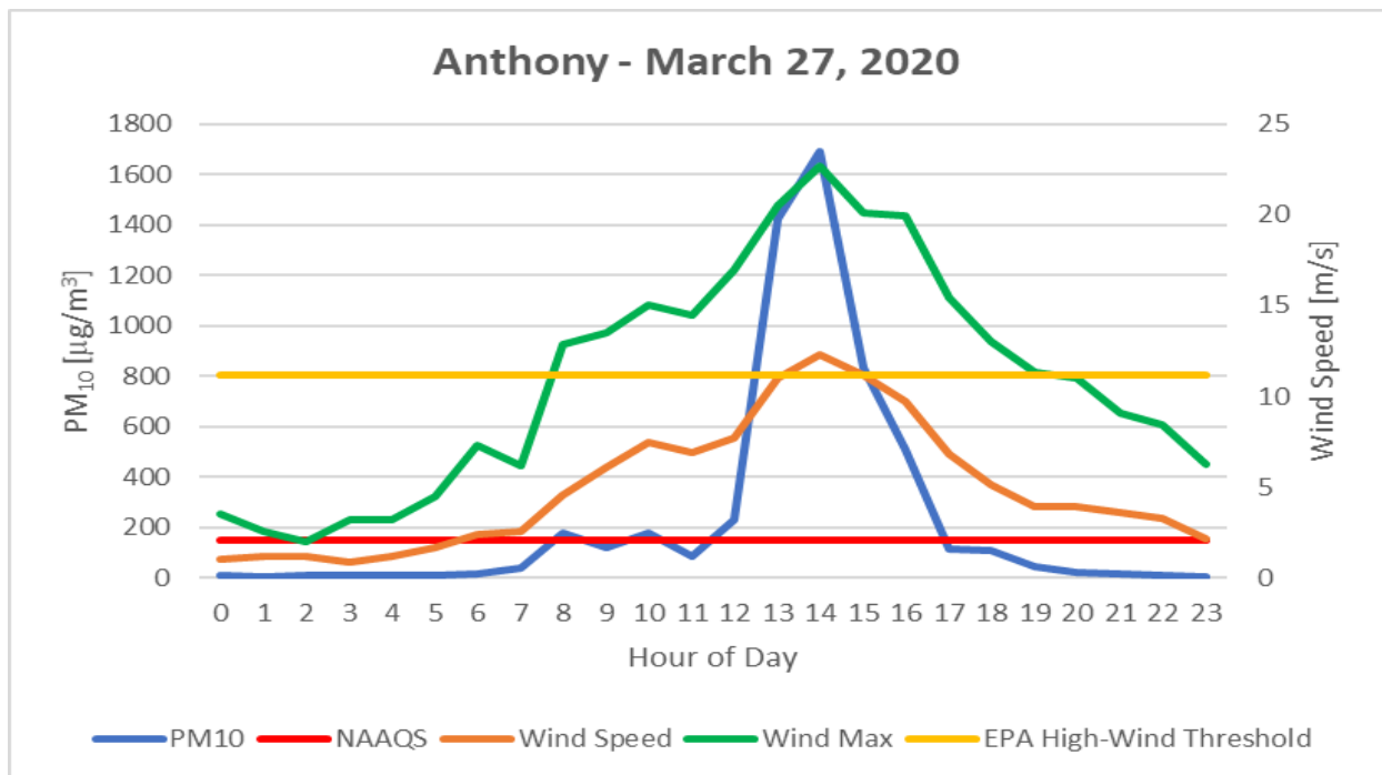
Figure 3-11. Anthony monitoring site hourly \text{PM}_{10} and wind speed data for the high wind blowing dust event.
