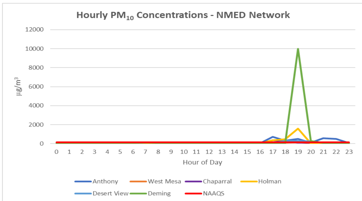
Figure 6-9. NMED monitoring network hourly PM 10 data for the high wind blowing dust event.
