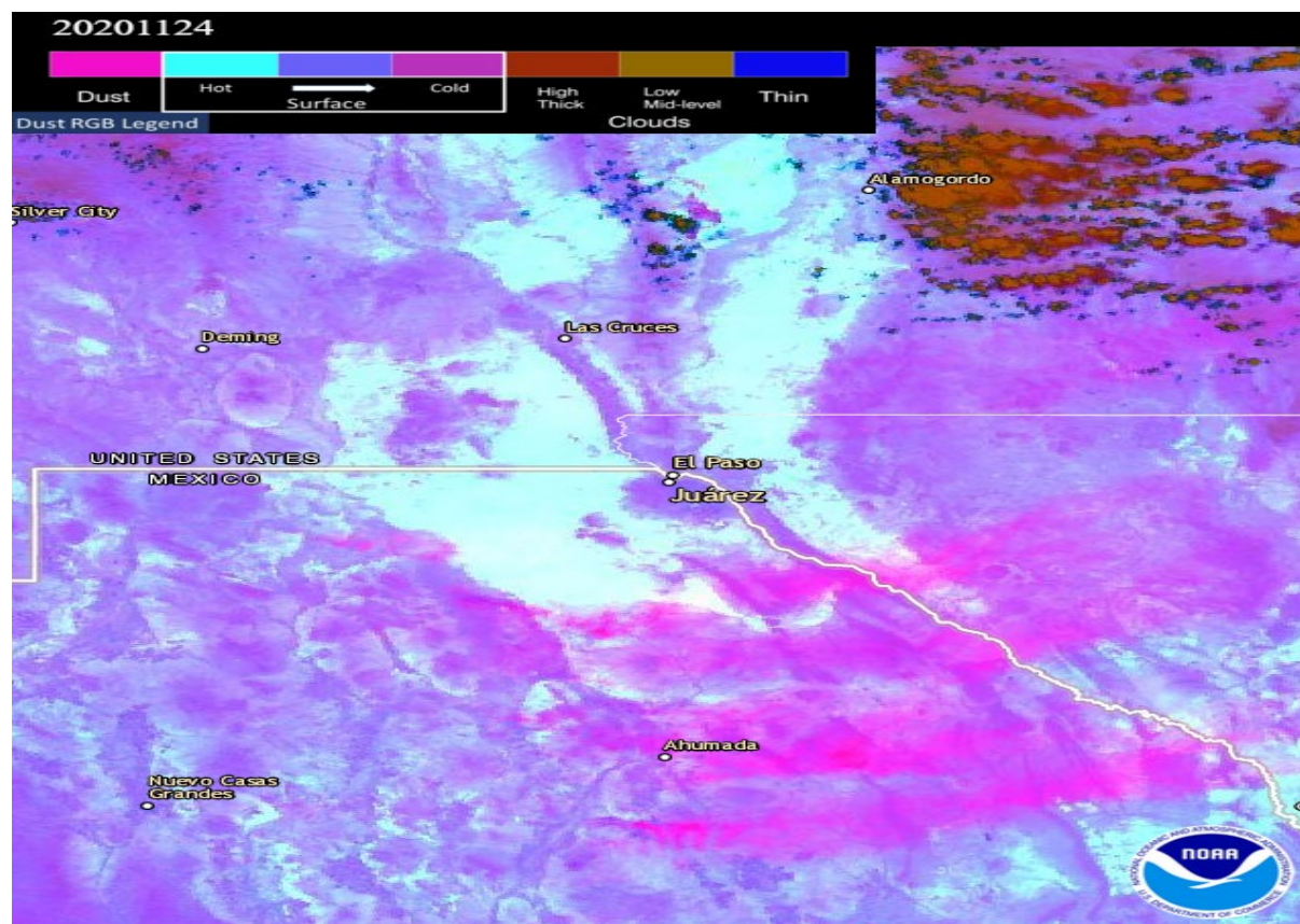
Figure 10-4. VIIRS RGB dust product from the NOAA-20 satellite showing southwestern New Mexico, northern Chihuahua and western Texas. Imagery obtained from NOAA's AerosolWatch website. Pink bands represent dust plumes.
