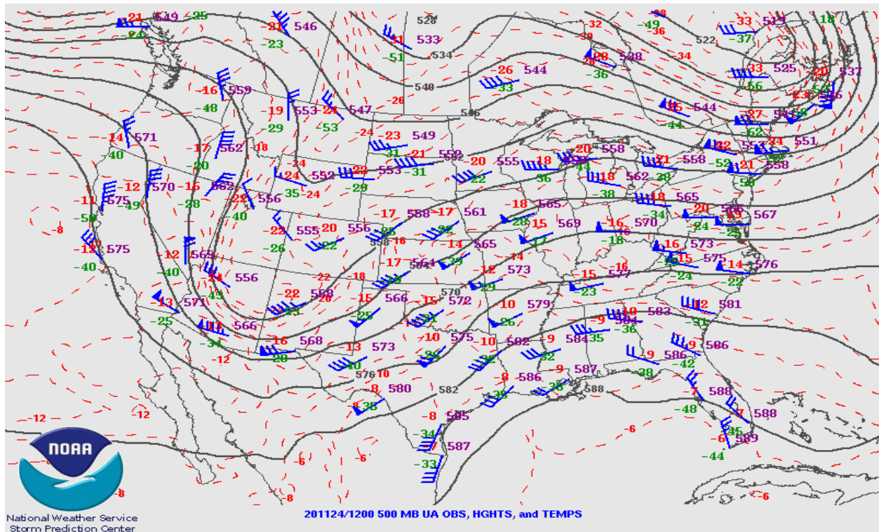
Figure 10-2. Upper air weather map for November 24, 2020 at the 1200 hour. Wind barbs depict wind speed (knots) and direction.
