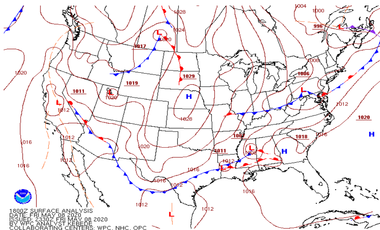
Figure 5-1. Surface weather map showing storm (surface low), cold fronts and isobars of constant pressure (red lines).
