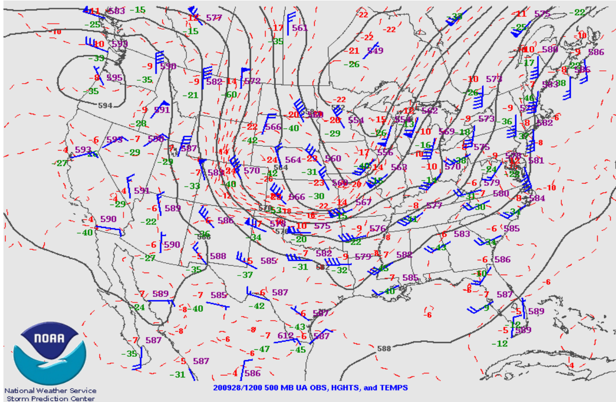
Figure 8-2. Upper air weather map for September 28, 2020 at the 1200 hour. Wind barbs depict wind speed (knots) and direction.
