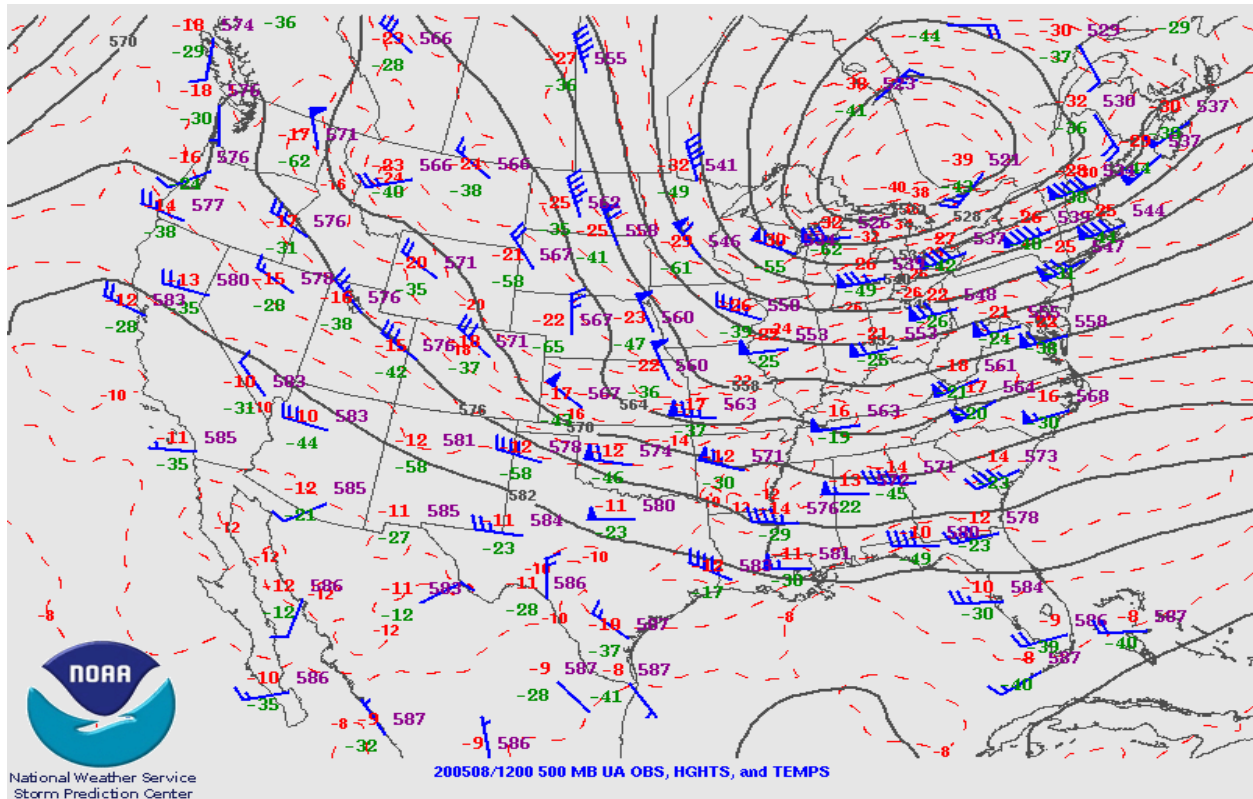
Figure 5-2. Upper air weather map for May 8, 2020 at the 1200 hour. Wind barbs depict wind speed (knots) and direction.
