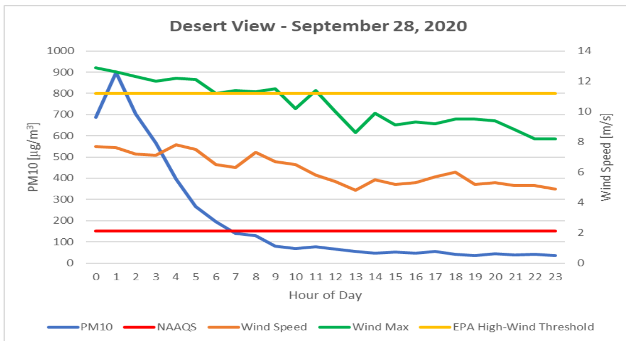
Figure 8-13. Desert View monitoring site hourly PM 10 and wind speed data for the high wind blowing dust event.
