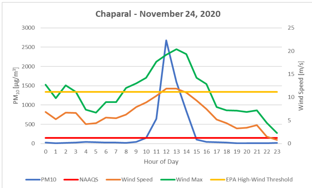
Figure 10-8. Chaparral monitoring site hourly PM 10 and wind speed data for the high wind blowing dust event.
