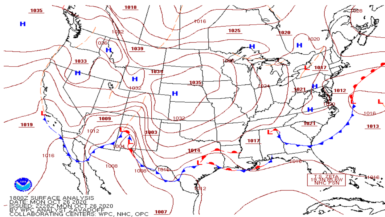
Figure 9-1. Surface weather map showing storm (surface low), cold fronts and isobars of constant pressure (red lines).
