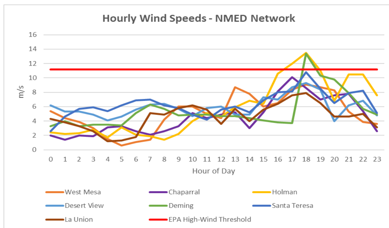
Figure 6-4. Wind speeds at NMED monitoring sites in Doña Ana and Luna Counties.
