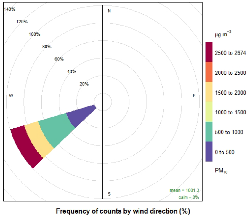
Figure 10-6. Pollution rose for the Chaparral monitoring site.
