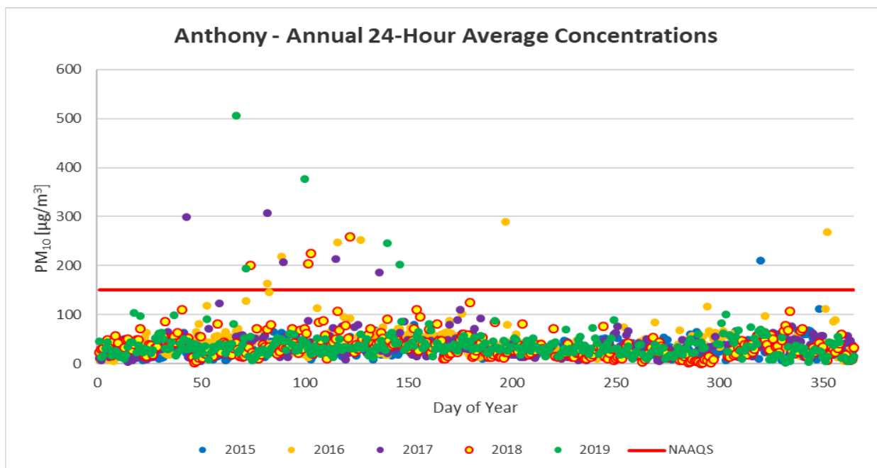
Figure 5-8. 24-hour averages by day of year from 2015-2019 for the Anthony monitoring site.
