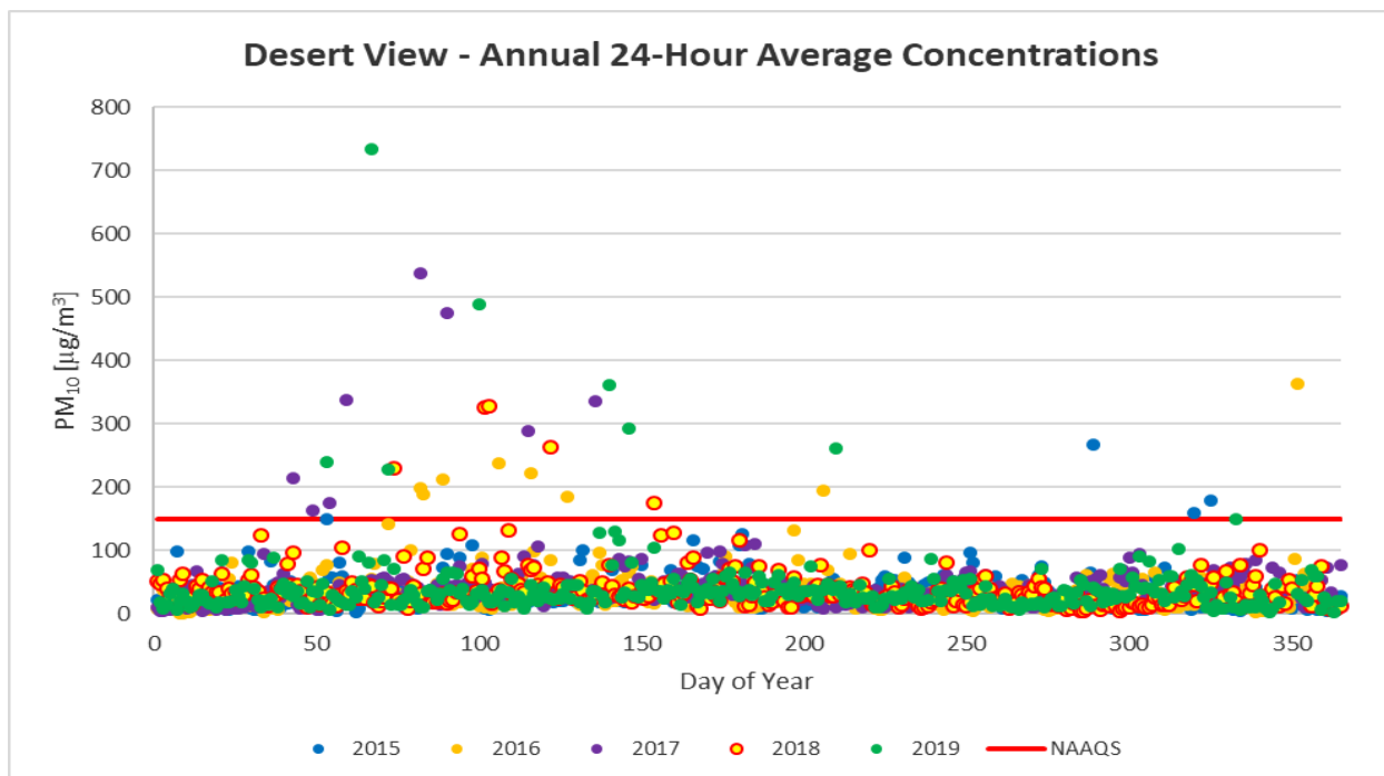
Figure 8-16. 24-hour averages by day of year from 2015-2019 for the Desert View monitoring site.
