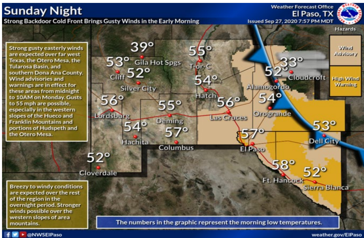
Figure 8-3. NWS Graphiccast product
