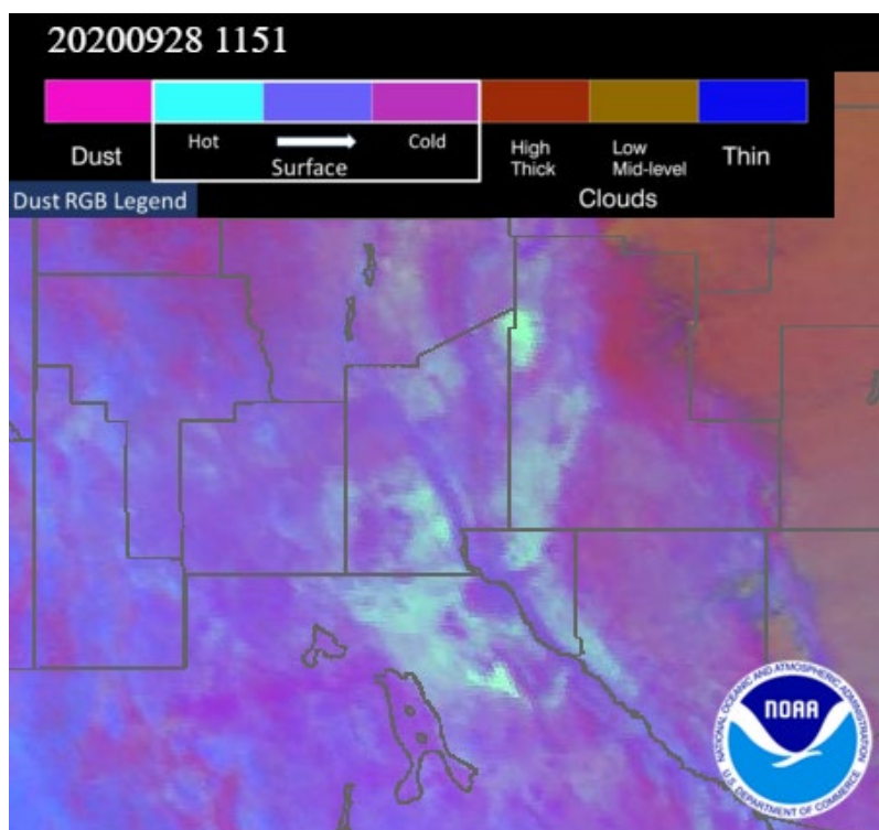
Figure 8-5. VIIRS Suomi NPP satellite dust RGB product imagery showing southwestern New Mexico, northern Chihuahua and western Texas. Imagery obtained from NOAA AerosolWatch website. Note: Pink bands represent dust plumes.
