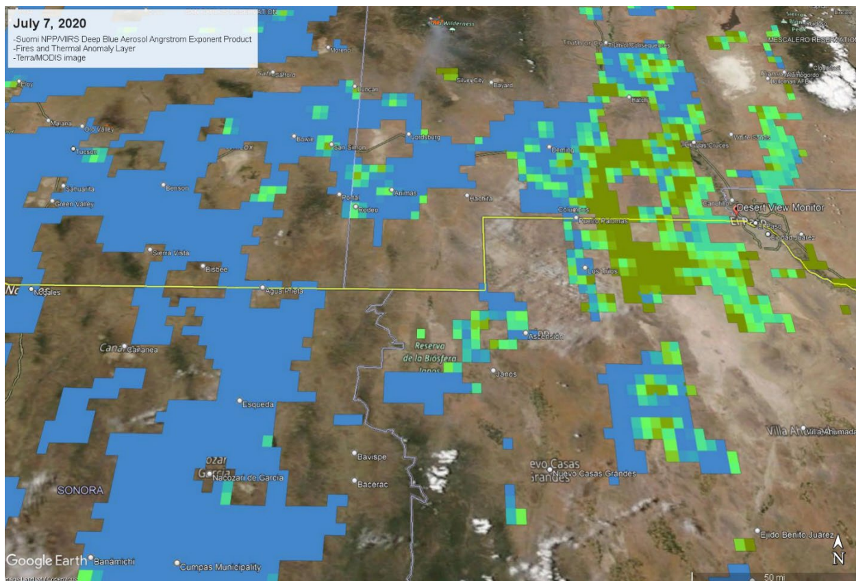
Figure-12-7. Suomi NPP/VIIRS Deep Blue Aerosol Angstrom Exponent Product showing smoke (blue) and dust (green) air columns July 7, 2020 for Southwestern New Mexico at 13:06 (MST). Image taken from Terra/MODIS satellite overhead pass at 10:35 (MST).
