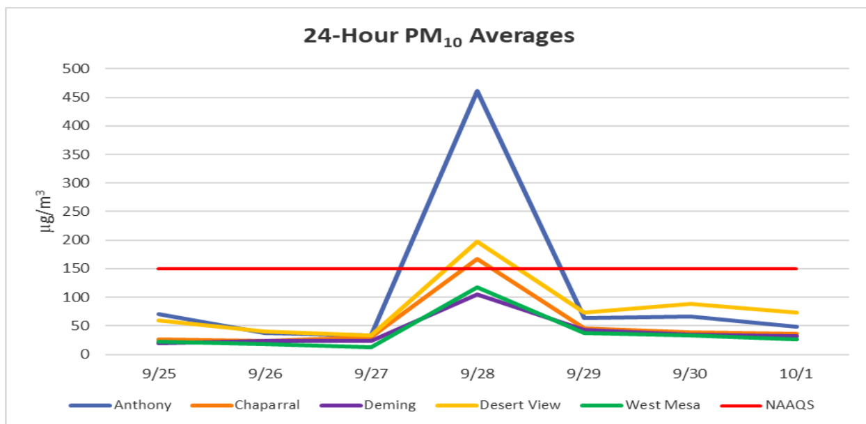
Figure 8-17. 24-Hour PM_{10} averages recorded at NMED monitoring sites for the event day and three days before and after.
