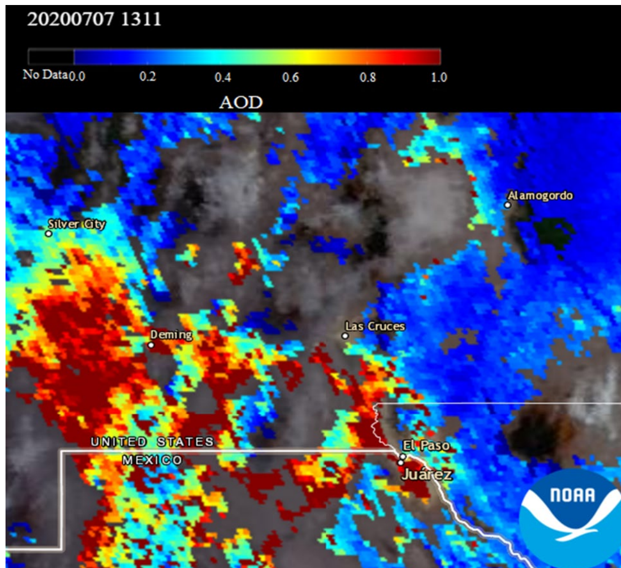
Figure -12-4. GOES-16 Aerosol Optical Depth Product at 06:11 (MST) showing southern Doña Ana and Luna Counties. Obtained from NOAA AerosolWatch.
