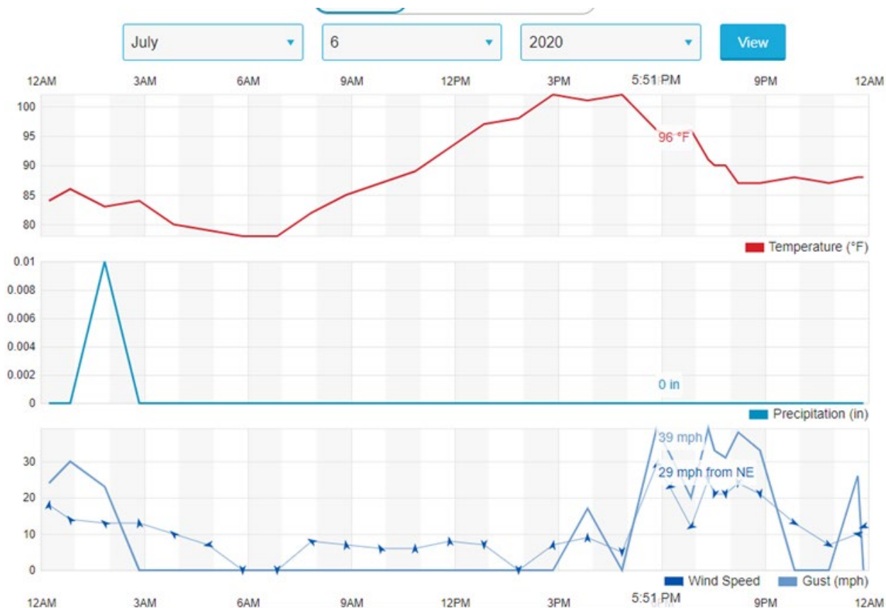
Figure 12-8. El Paso International wind speed data for July 6, 2020. Obtained from Weather Underground.
