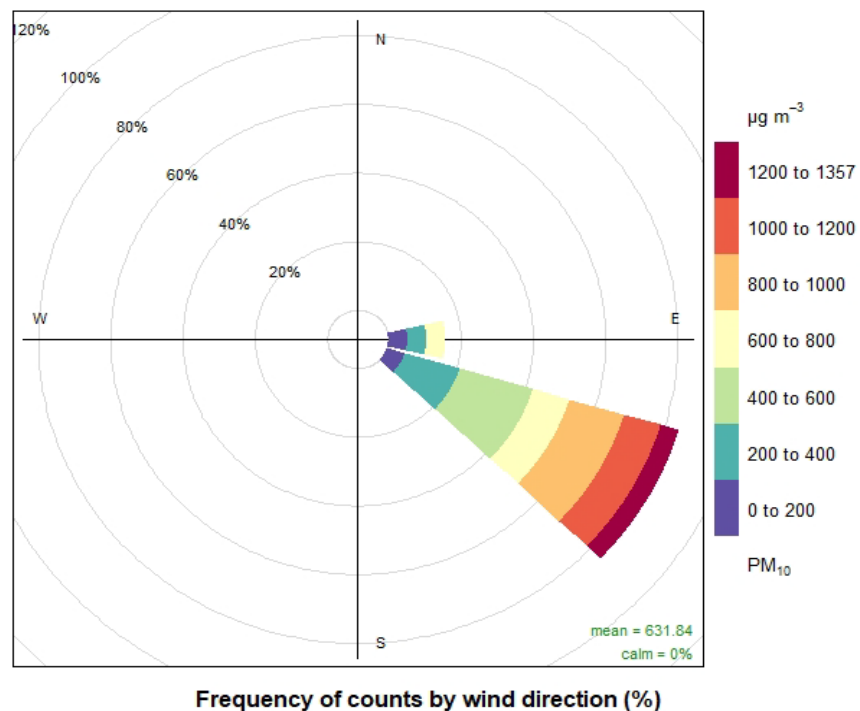
Figure 9-5. Pollution rose for the Desert View monitoring site
