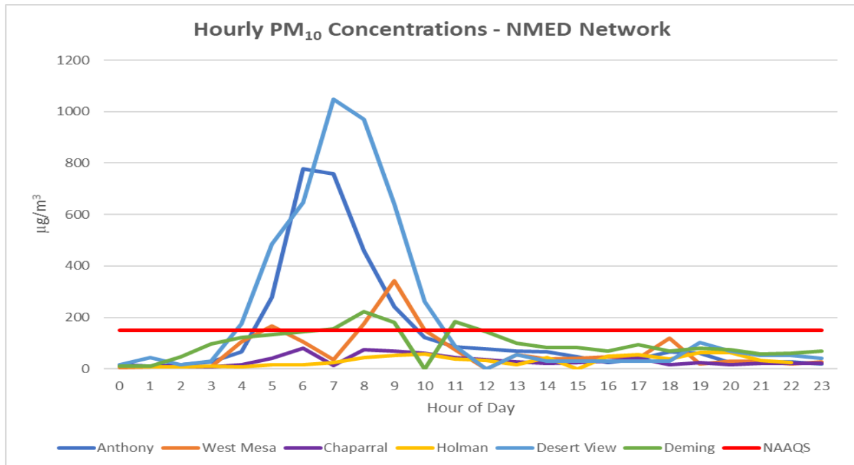
Figure 7-8. NMED monitoring network hourly PM 10 data for the high wind blowing dust event.
