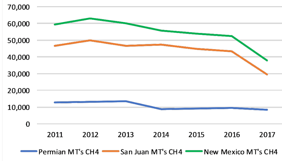
NM equipment leak methane emissions
