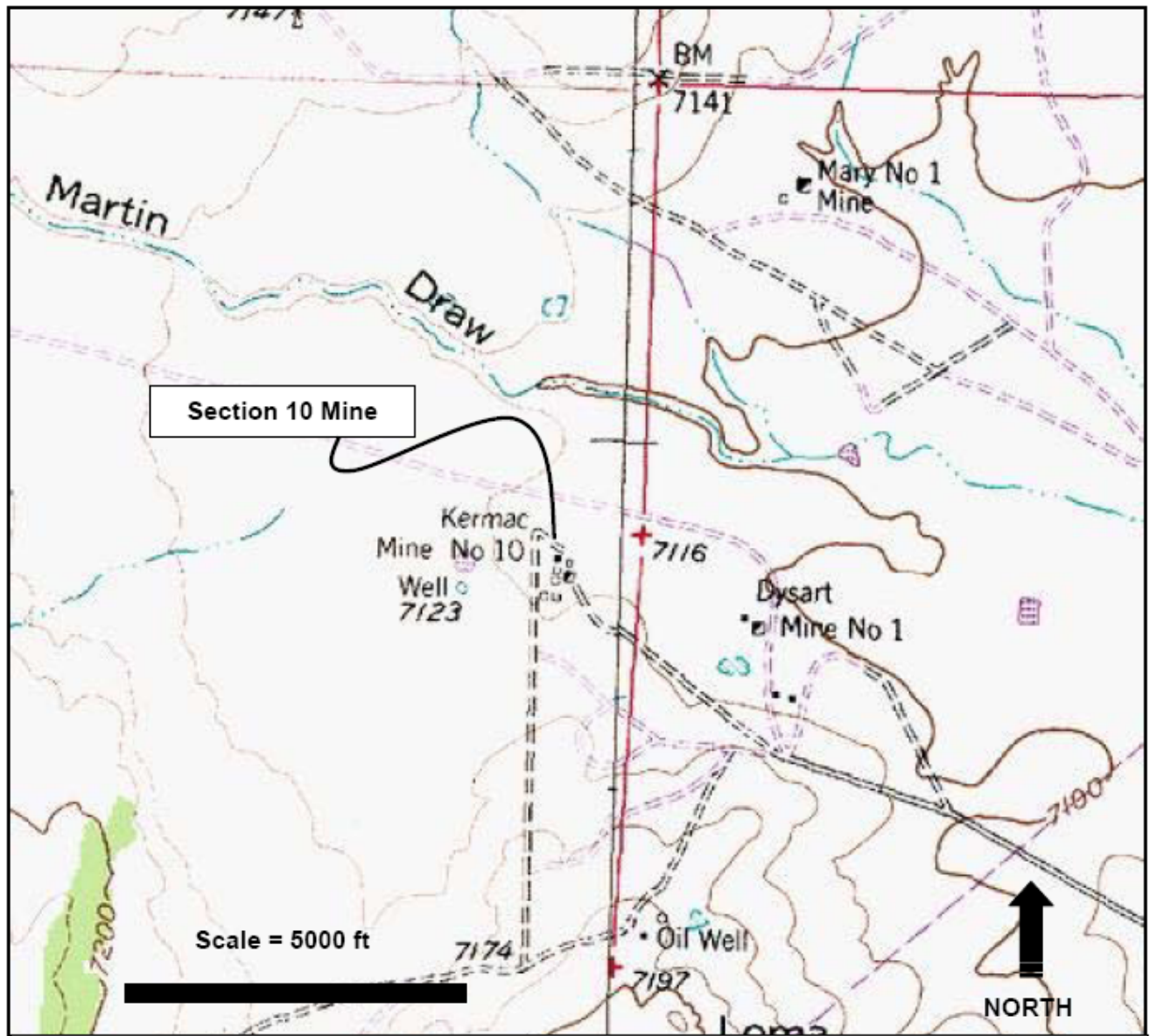
Figure 2. TopoQuest.com location map of the Section 10 Mine in USGS Goat Mountain 7.5 Minute Quadrangle, Ambrosia Lake Subdistrict, Grants, NM.
