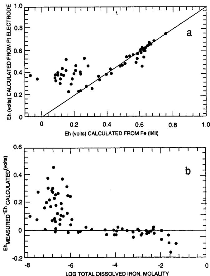
FIGURE 6.3—(a) Comparison of Eh calculated from the Fe (II/III) redox couple to Eh measured with a platinum electrode. (b) Difference between calculated and measured Eh plotted as function of total dissolved iron concentrations in molal units. Data from Leviathan/Bryant Creek watershed, California and Nevada (Ball and Nordstrom, 1989; 1994).
