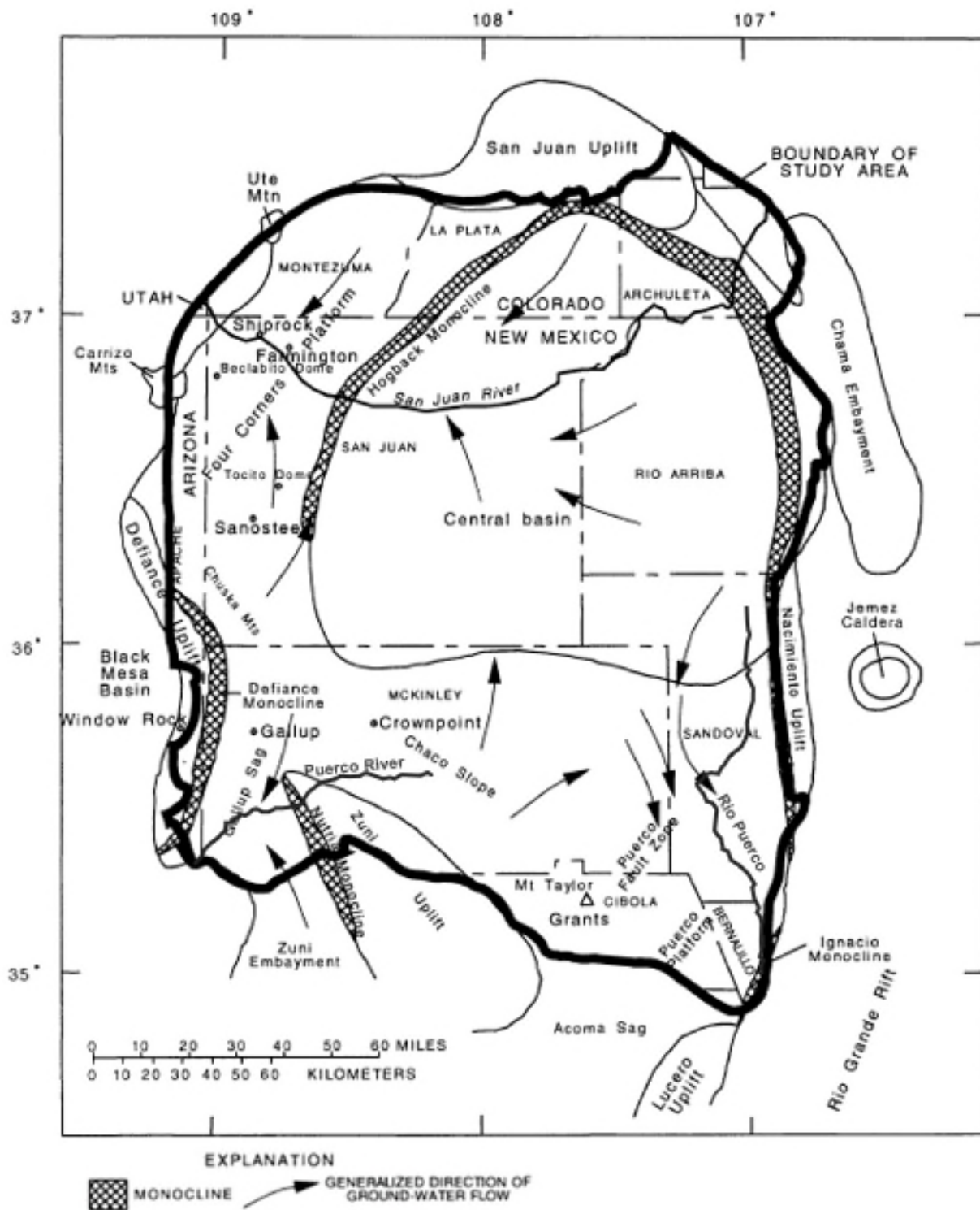
PEABODY EXHIBIT 16. Structural elements of the San Juan Basin and generalized patterns of groundwater flow in Jurassic and Cretaceous age bedrock (modified from Dam, 1995)
